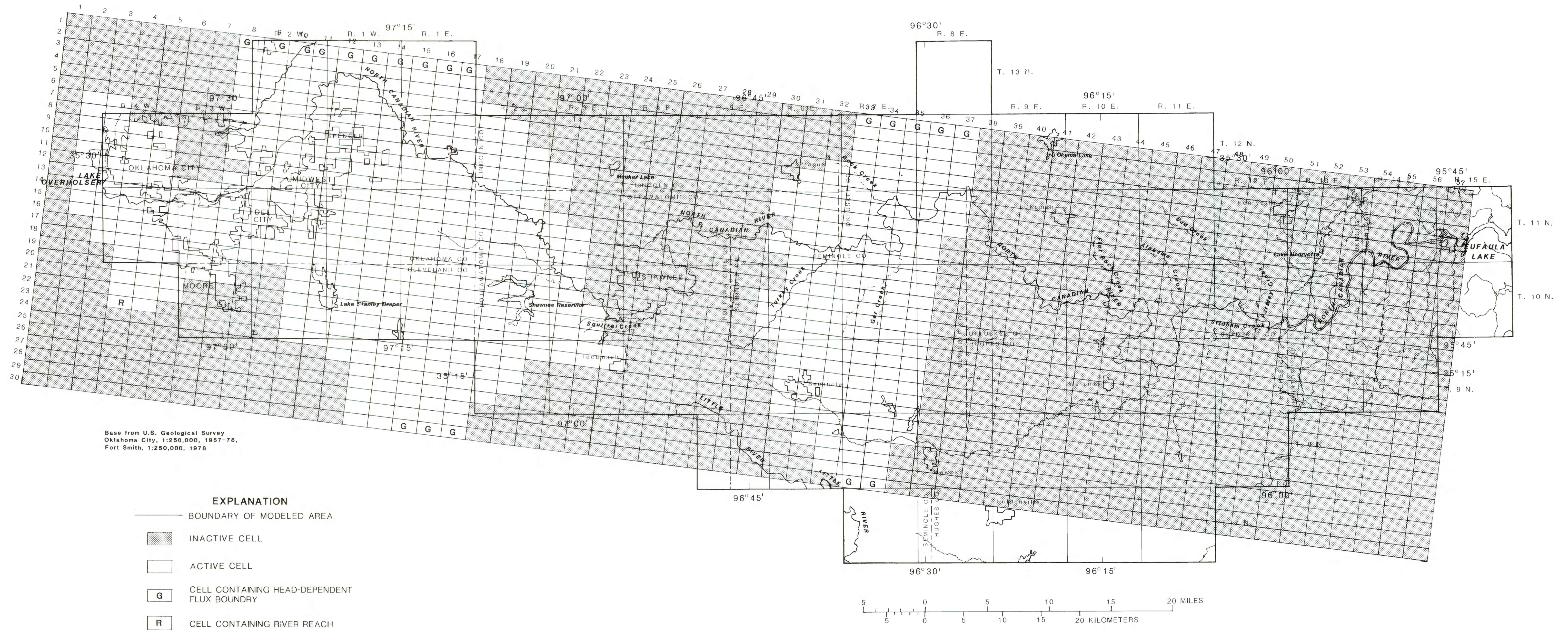
FINITE-DIFFERENCE GRID OF GARBER-WELLINGTON AND ADA-VAMOOSA AQUIFERS, EAST-CENTRAL OKLAHOMA
