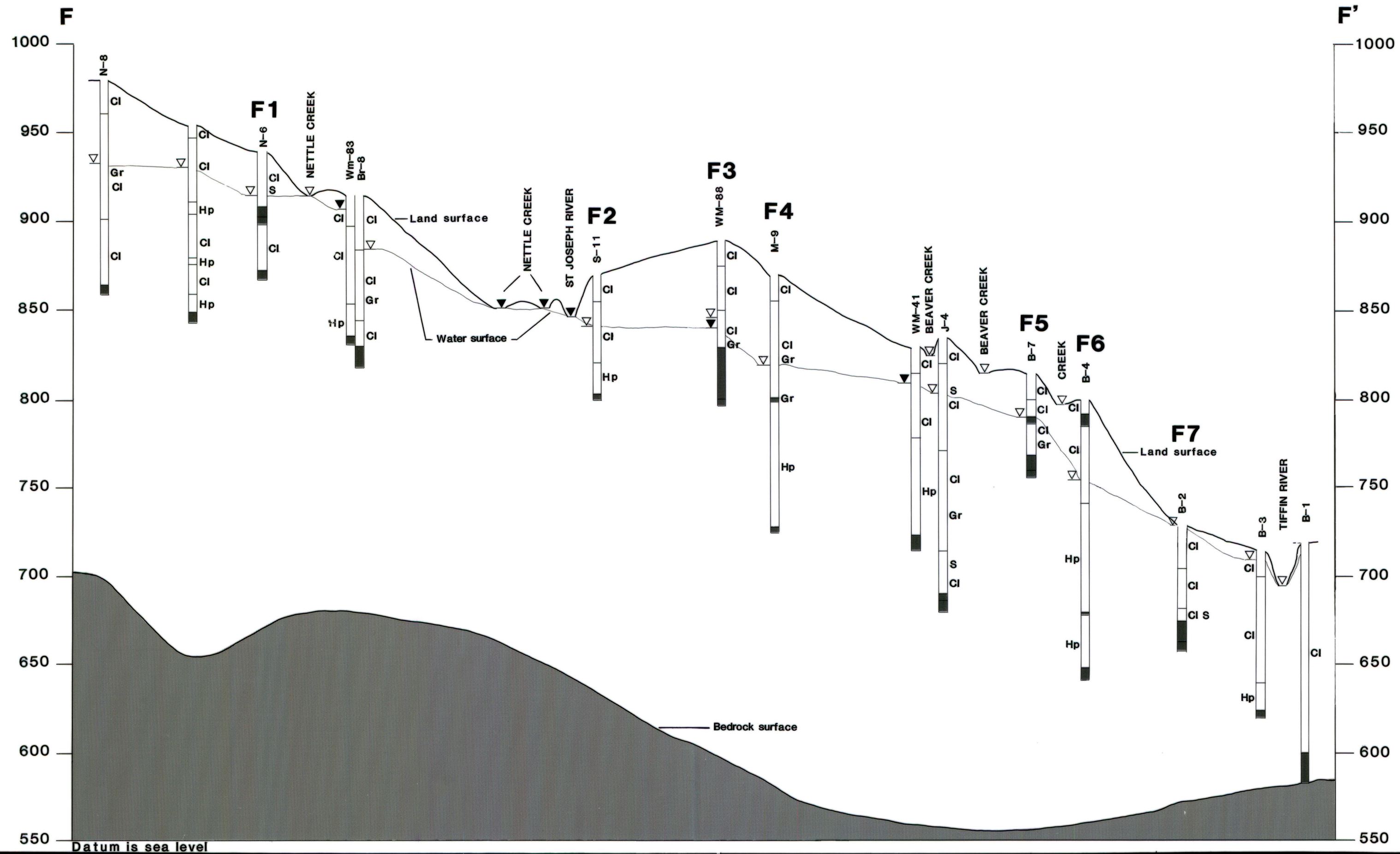
Figure 9.—Generalized geological sections through Williams County, Ohio—Continued.
