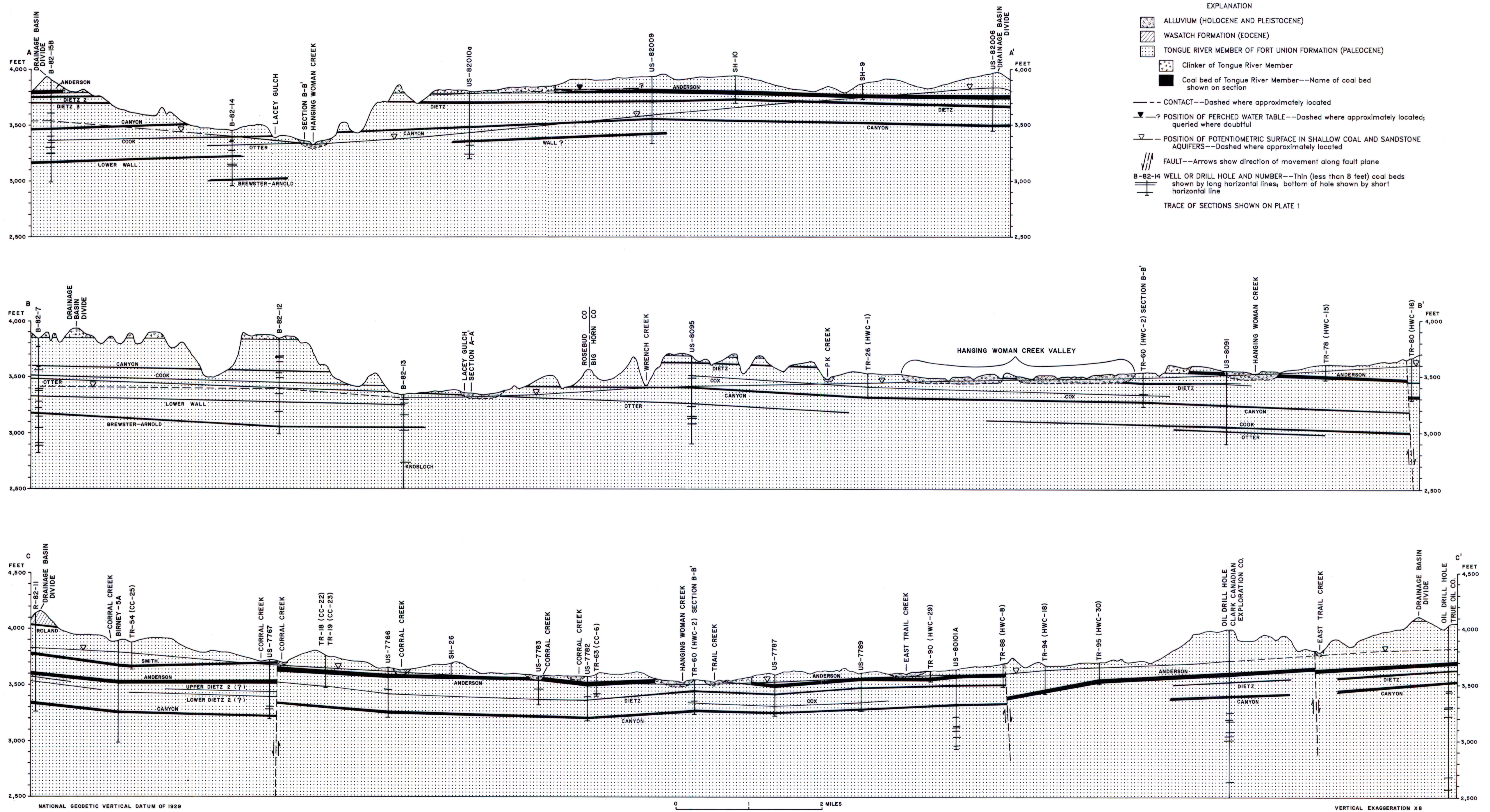
IDEALIZED HYDROGEOLOGIC SECTIONS A-A', B-B', AND C-C' IN THE HANGING WOMAN CREEK BASIN, SOUTHEASTERN MONTANA
