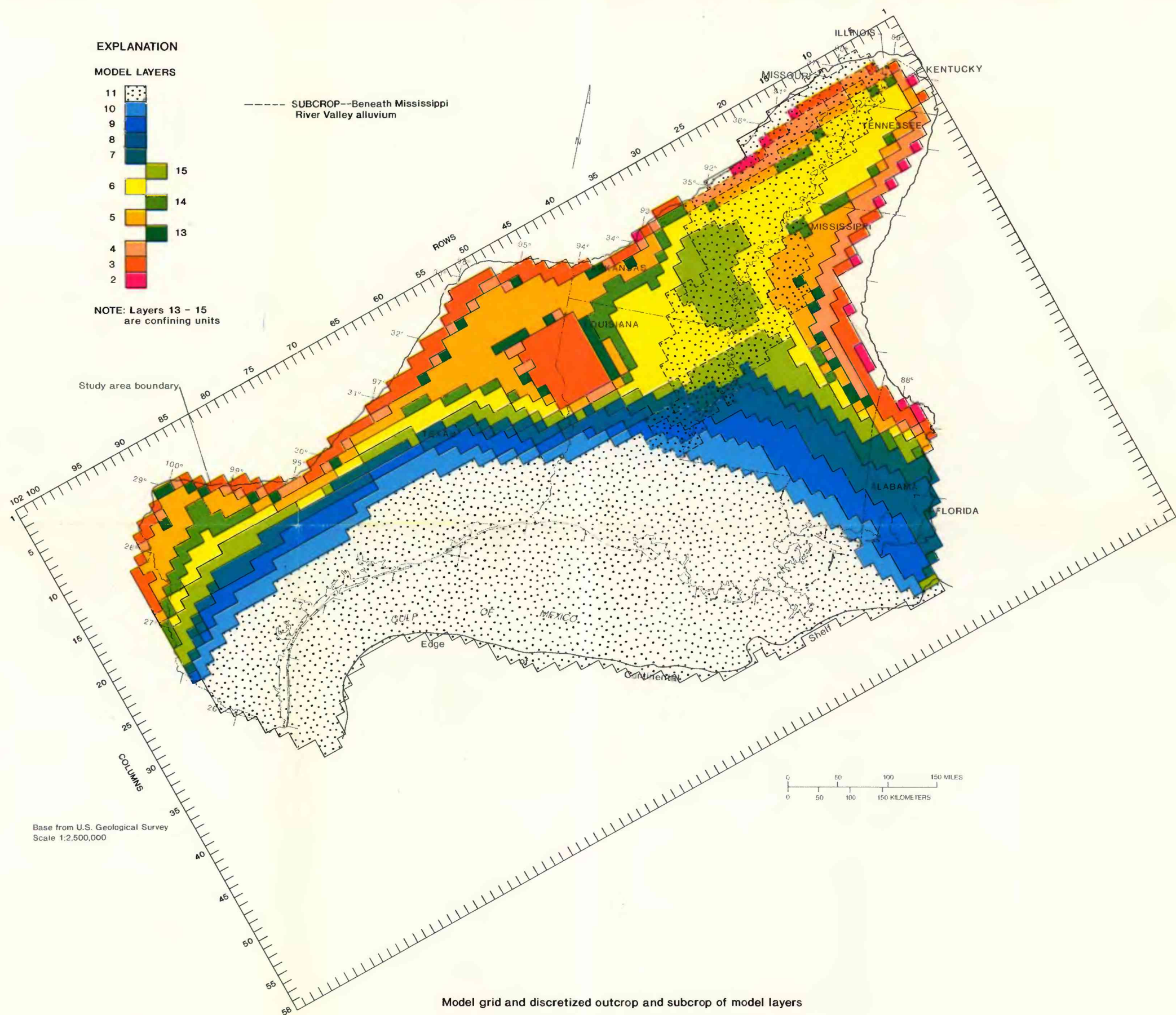
GROUND-WATER FLOW IN THE GULF COAST AQUIFER SYSTEMS, SOUTH-CENTRAL UNITED STATES--A PRELIMINARY ANALYSIS
