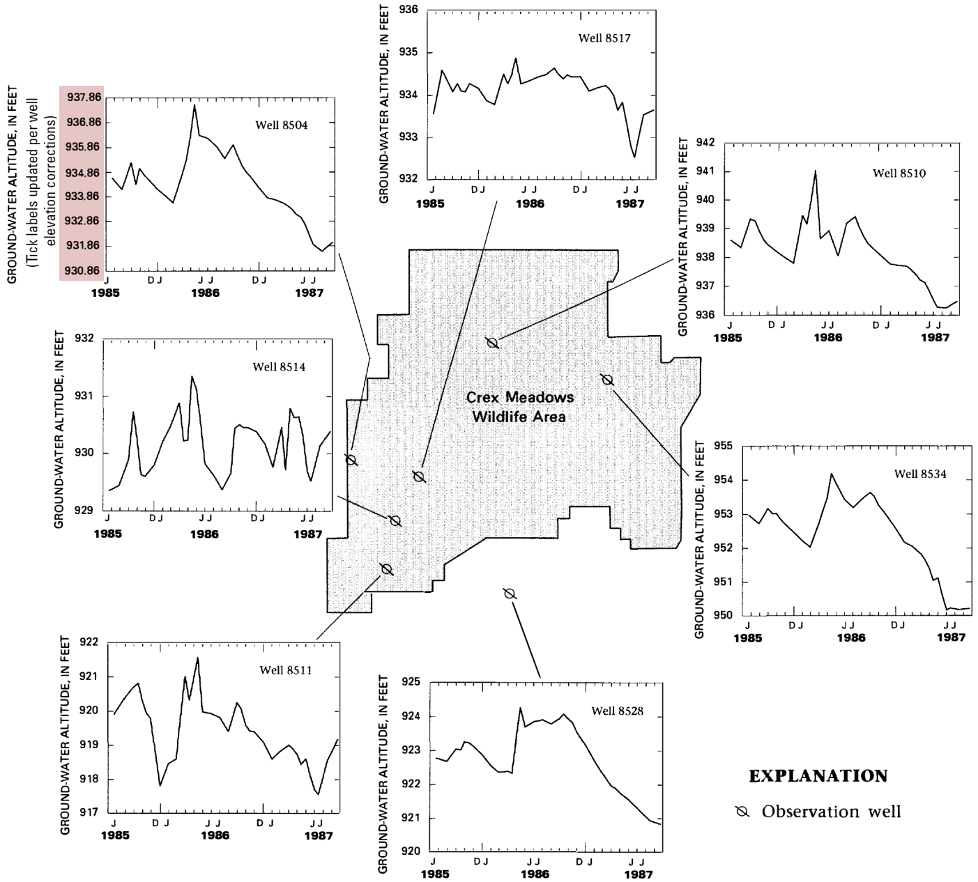
Figure 6. Ground-water levels at selected wells in the Crex Meadows area.
