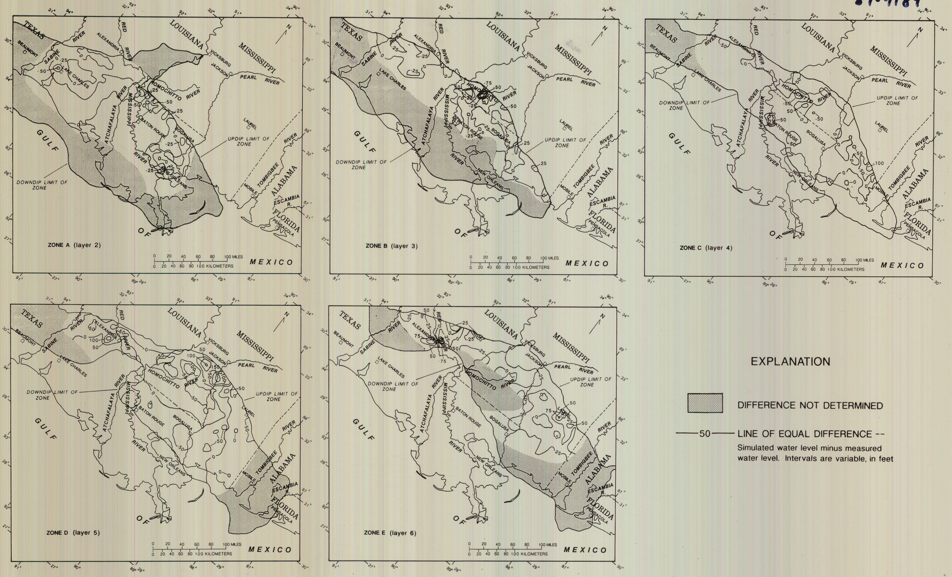
Figure 5.--The differences between model-simulated and measured water-level altitudes for 1980.
