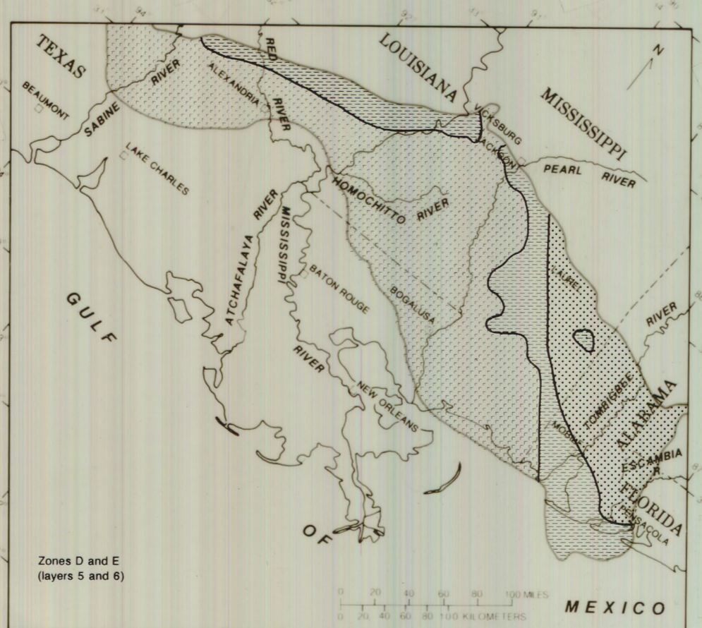
Figure 11.--Areal distribution of vertical leakance between the permeable zones in the calibrated model.
