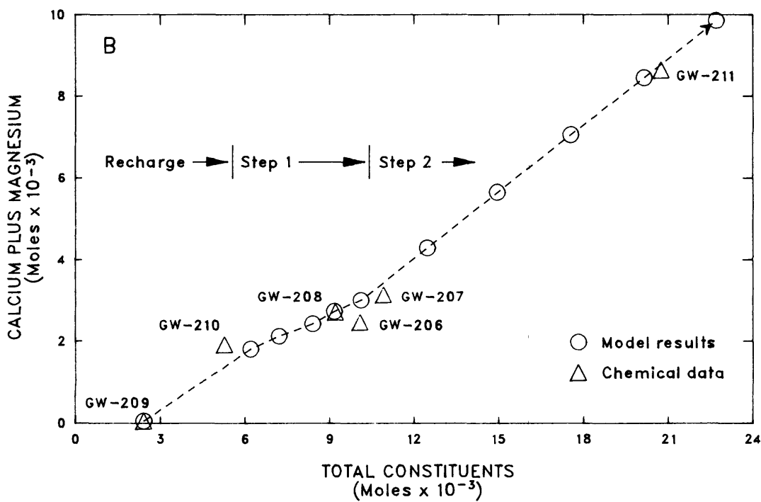
Figure 21.--(A) Chemical evolution of water in the Rome Formation from the PHREEQE model and (B) chemical analyses of water from selected wells. (Well locations shown on figure 3.)
