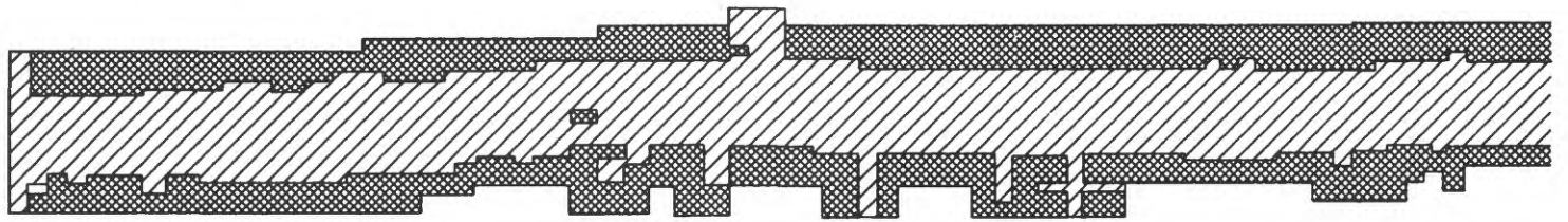
Layers 3 and 4
