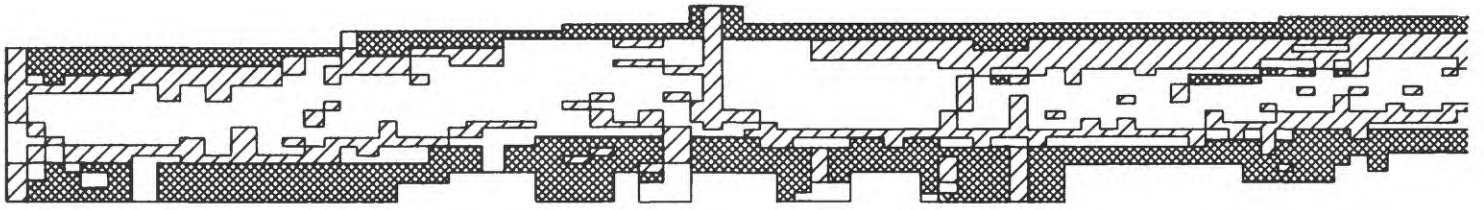
Layers 1 and 2
