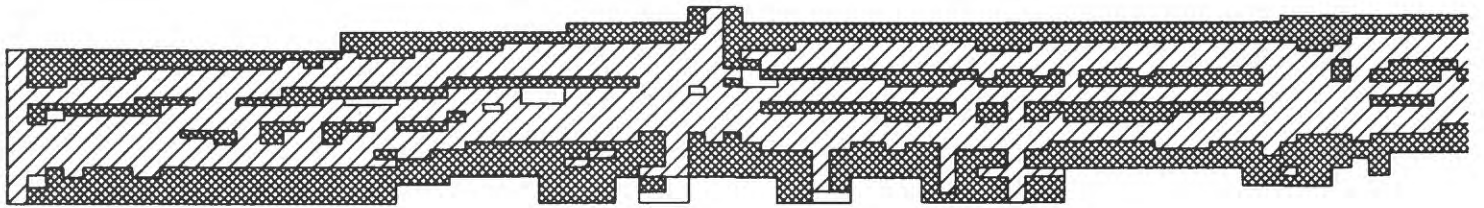
Layers 2 and 3
