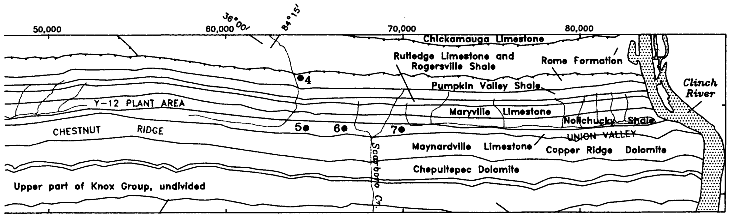
Figure 3.--Bedrock geology--Continued.
