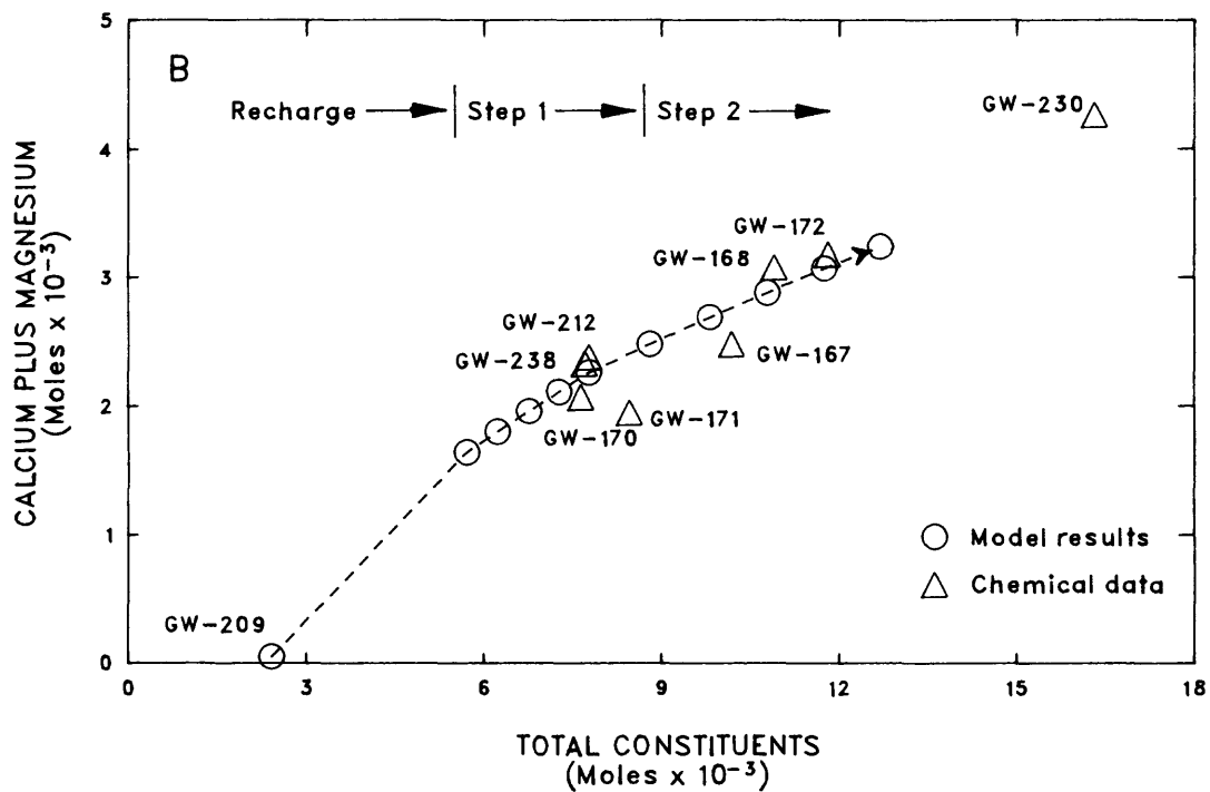
Figure 22.--(A) Chemical evolution of water in the Maynardville Limestone from the PHREEQE model and (B) chemical analyses of water from selected wells. (Well locations shown on figure 3.)
