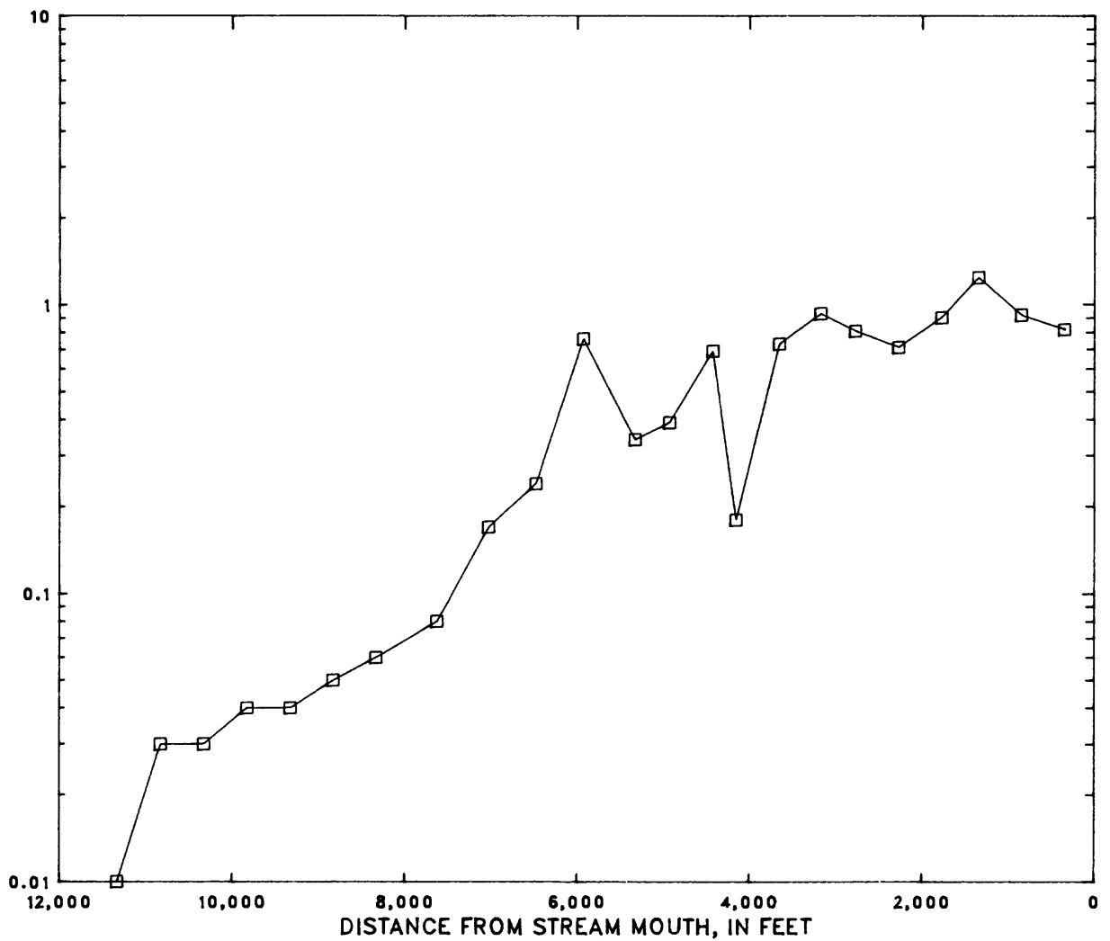
Figure 5.—Ground-water gains and losses and cumulative ground-water discharge along Scarboro Creek, March 10, 1984.
