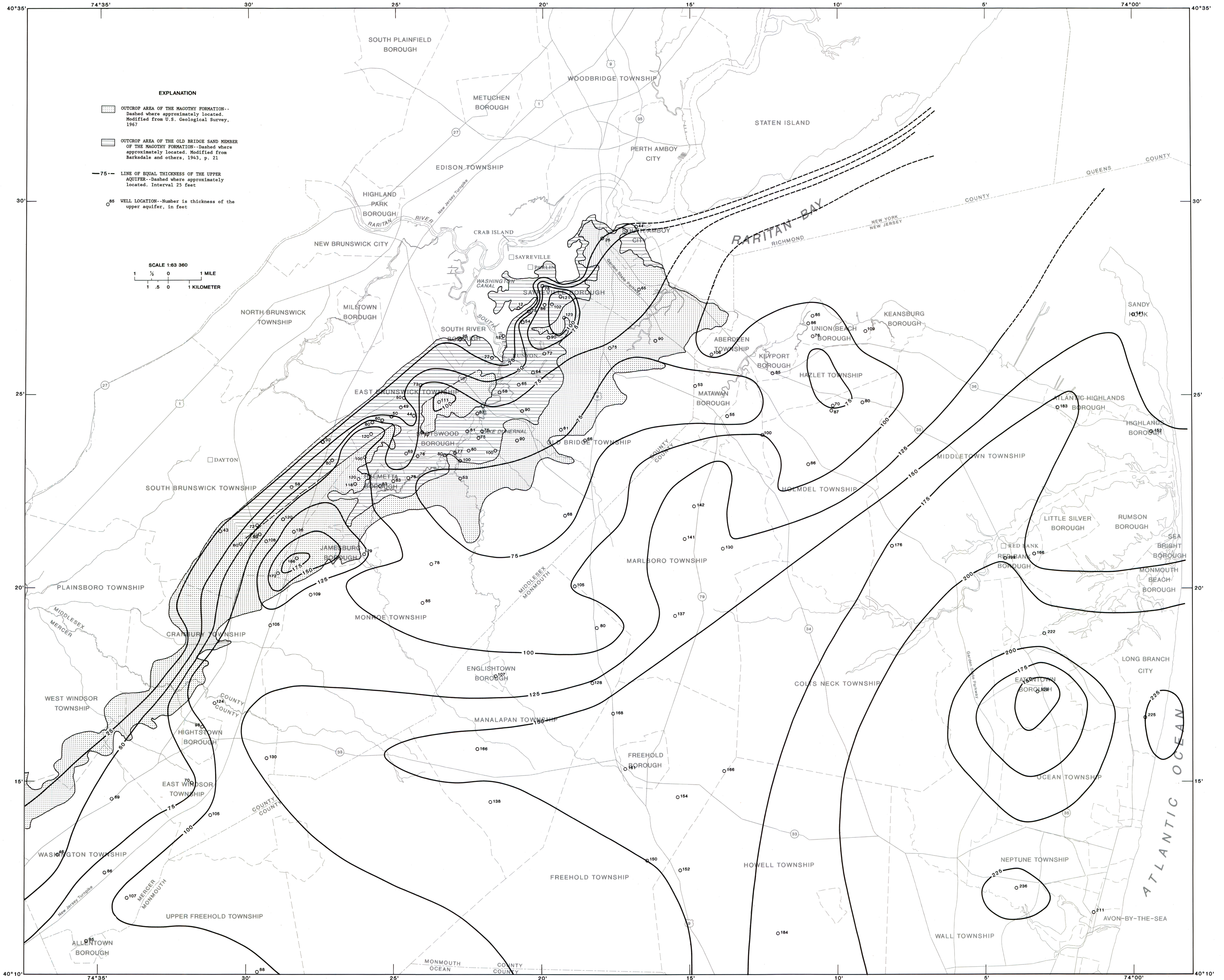
THICKNESS OF THE UPPER AQUIFER OF THE POTOMAC-RARITAN-MAGOTHY AQUIFER SYSTEM, NORTHERN COASTAL PLAIN, NEW JERSEY
