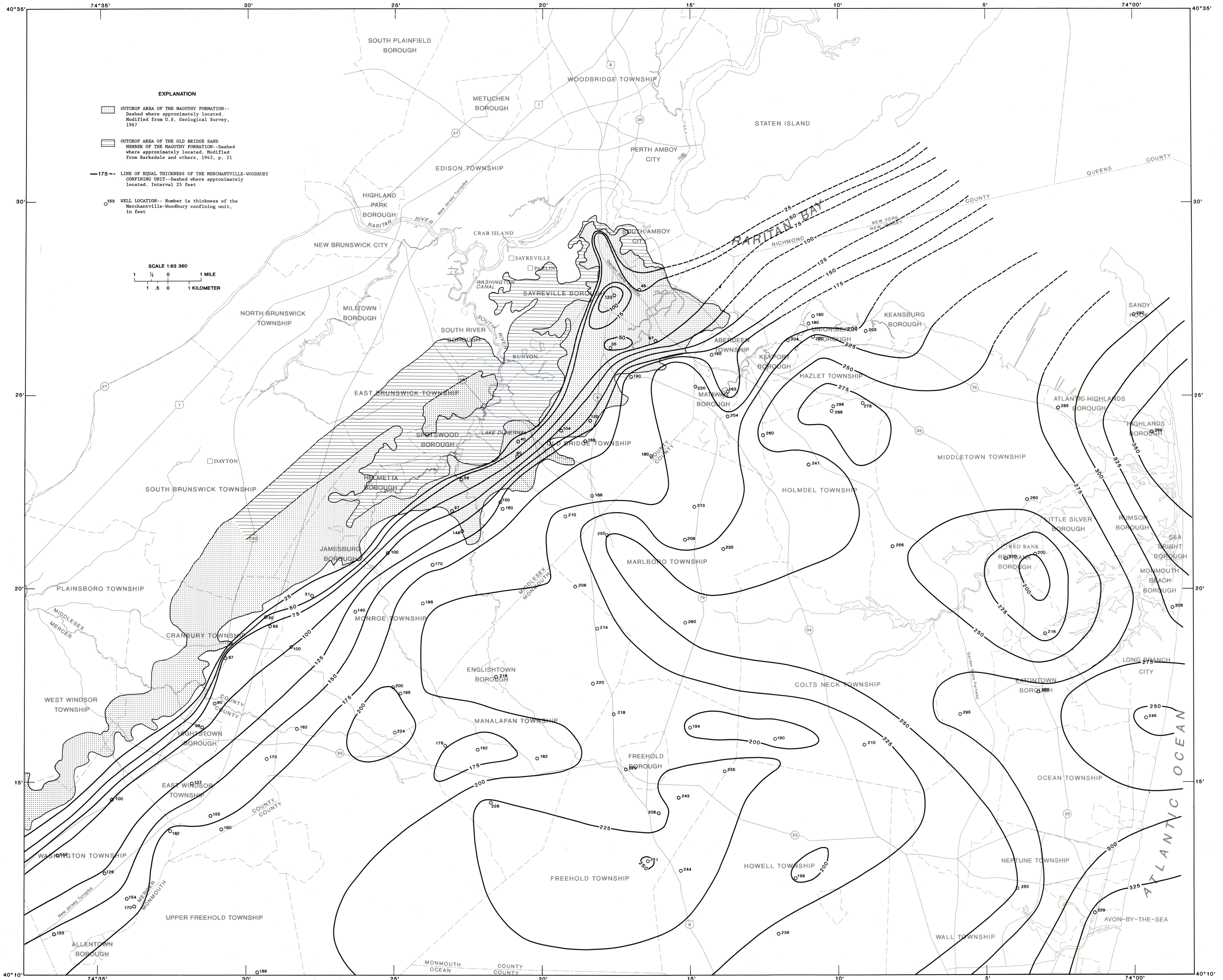
THICKNESS OF THE MERCHANTVILLE-WOODBURY CONFINING UNIT, NORTHERN COASTAL PLAIN, NEW JERSEY
