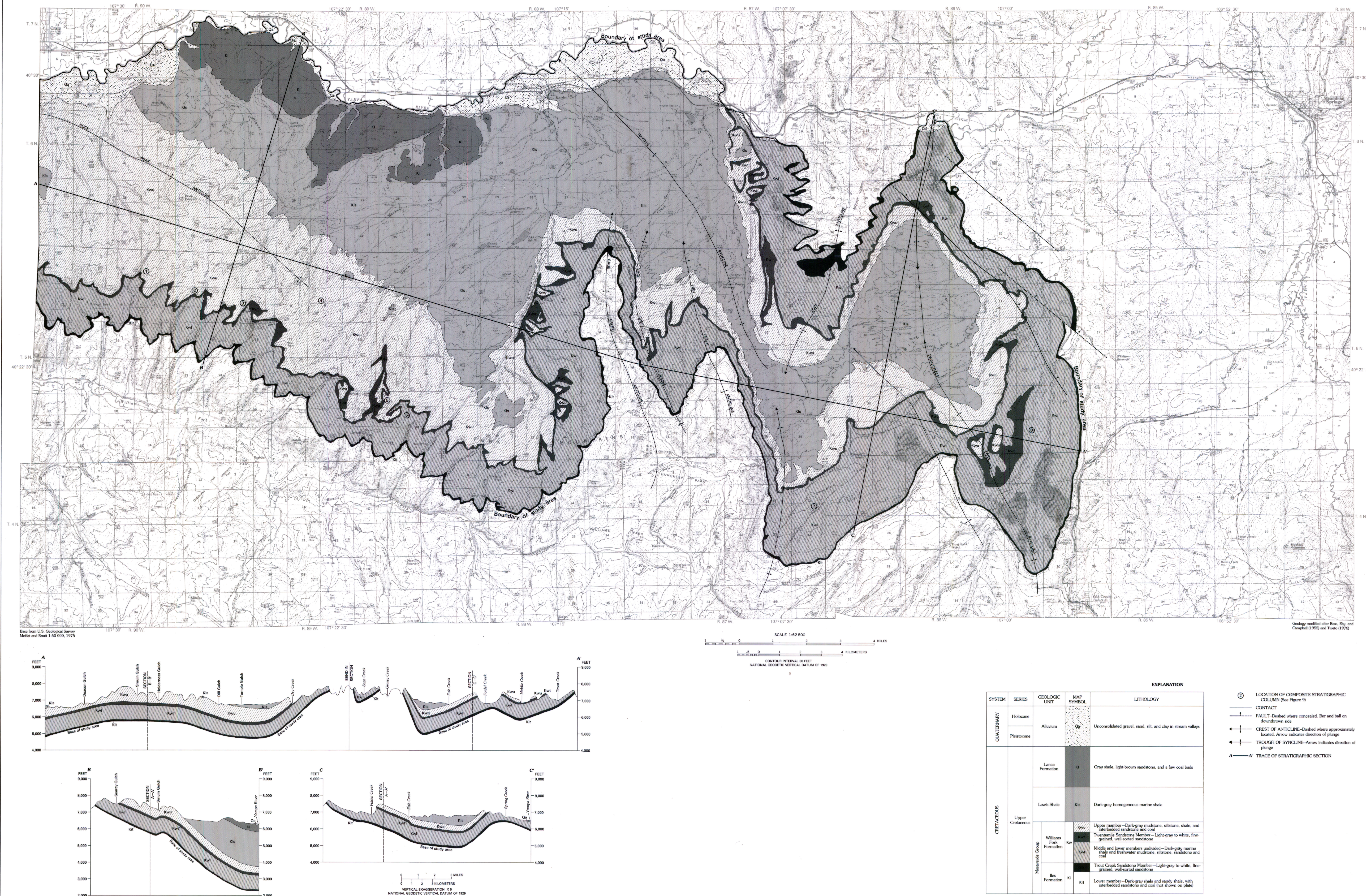
MAP SHOWING GEOLOGY AND GENERALIZED STRATIGRAPHIC SECTIONS IN NORTHWESTERN COLORADO
