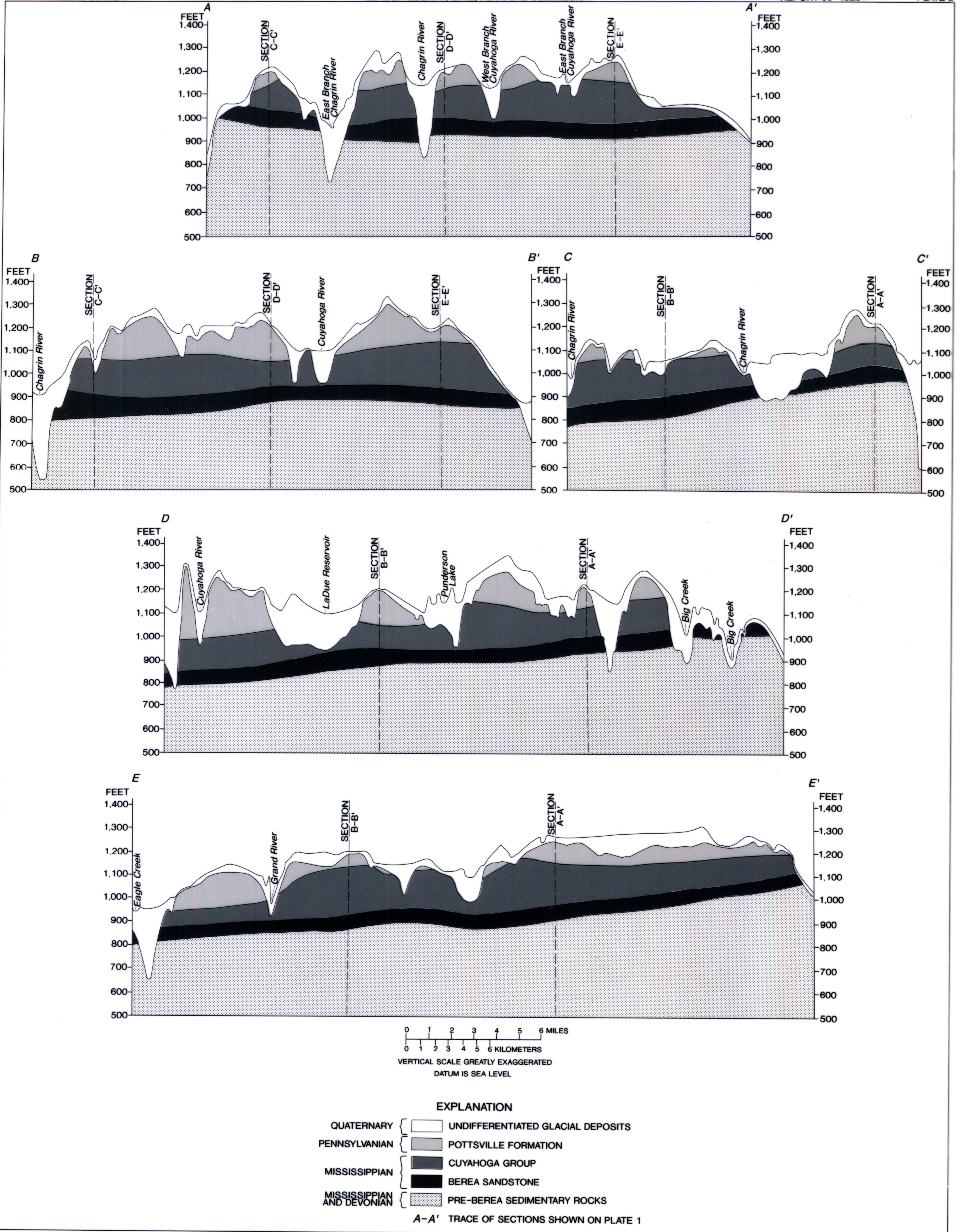
GENERALIZED GEOLOGIC SECTIONS OF GEAUGA COUNTY, OHIO
