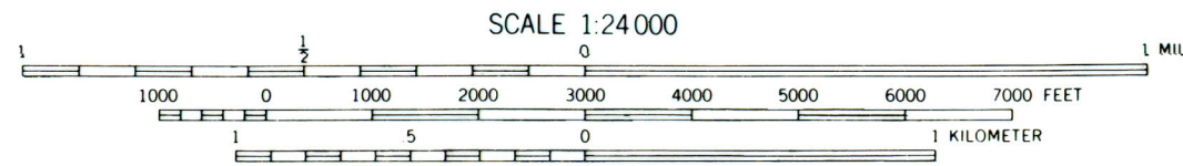
DEPTH TO BEDROCK SURFACE, RAMAPO RIVER VALLEY, NEW JERSEY AND NEW YORK
