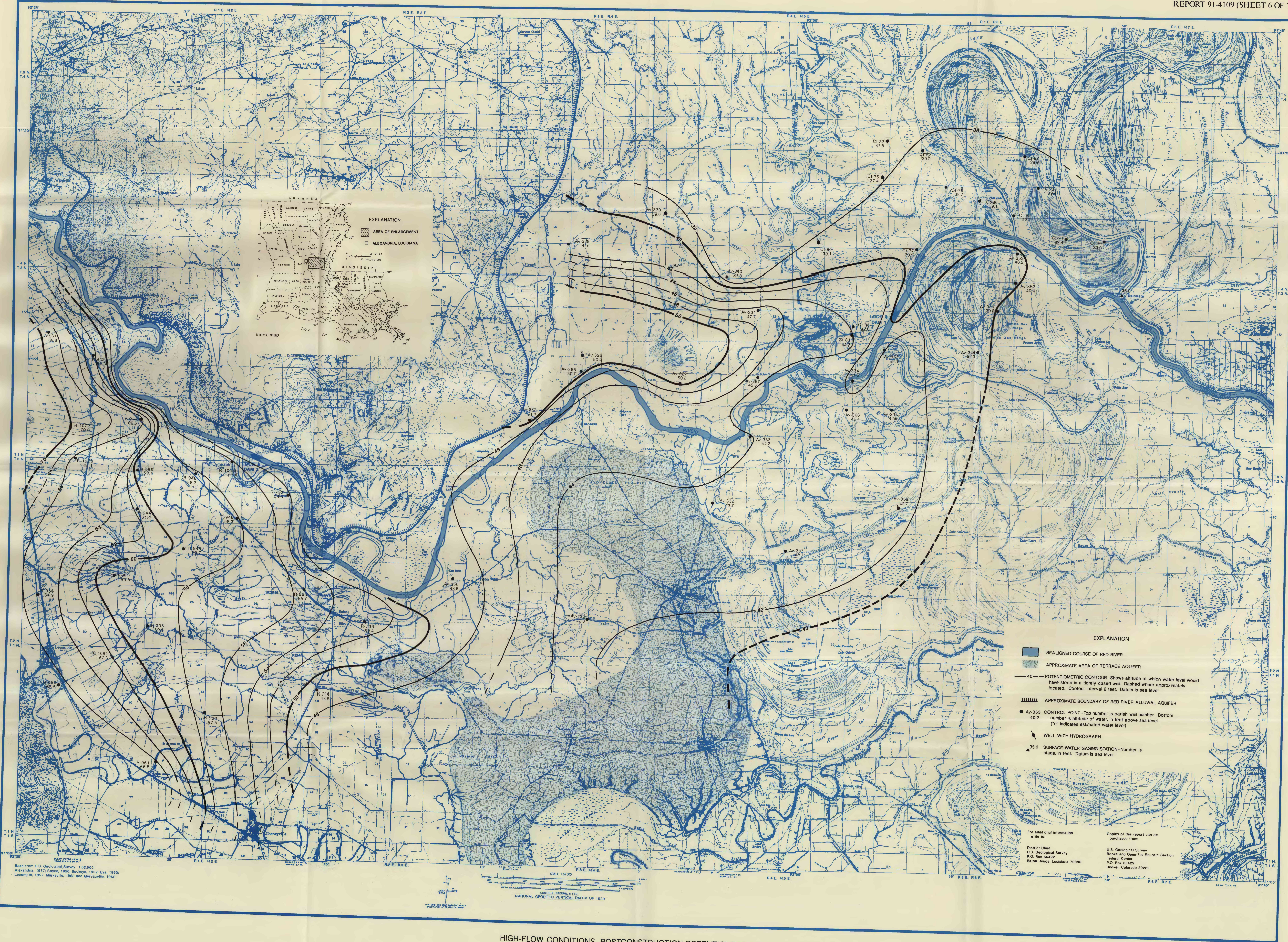
HIGH-FLOW CONDITIONS, POSTCONSTRUCTION POTENTIOMETRIC SURFACE, APRIL 1987
