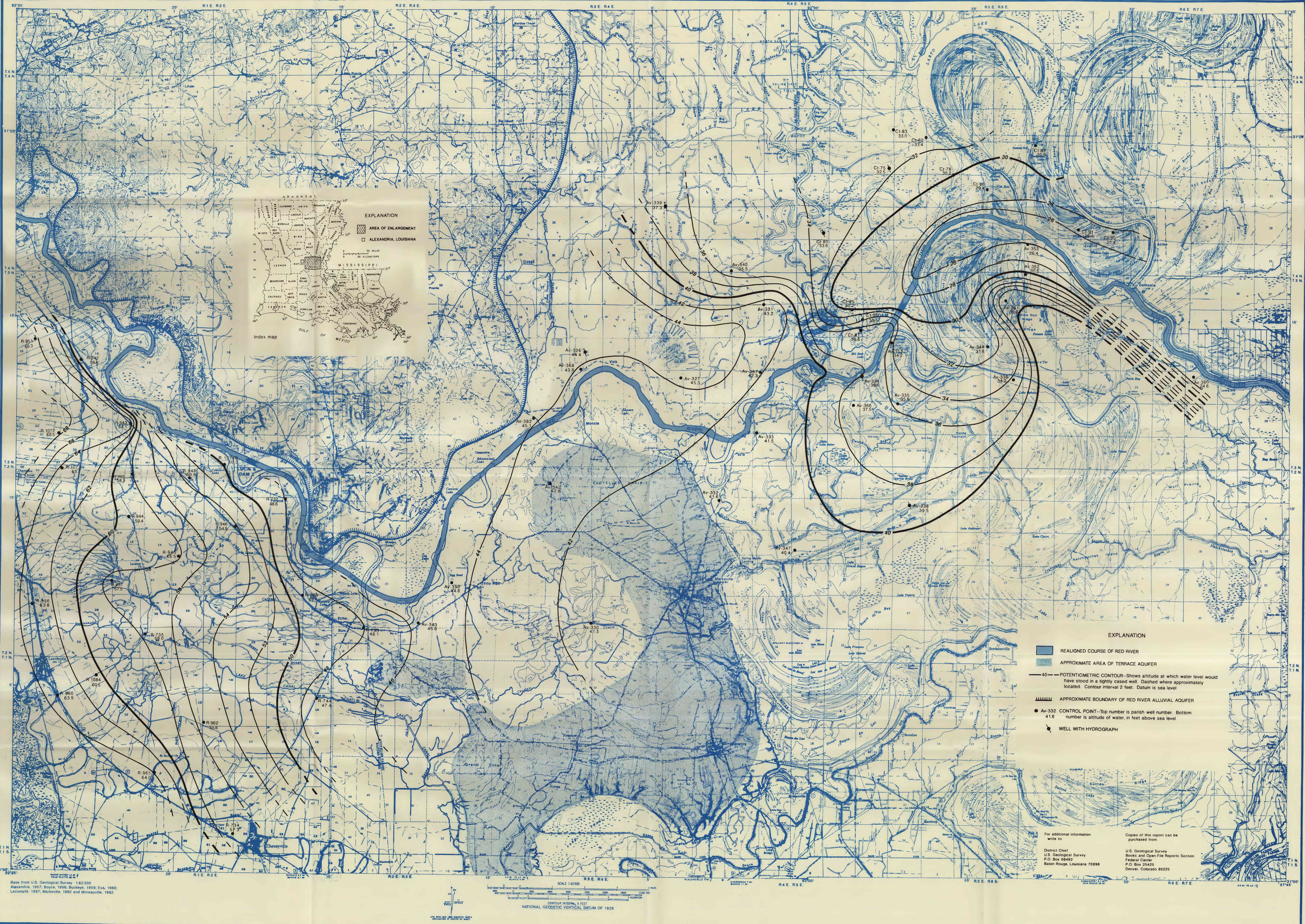
AVERAGE POSTCONSTRUCTION POTENTIOMETRIC SURFACE, 1985-87
