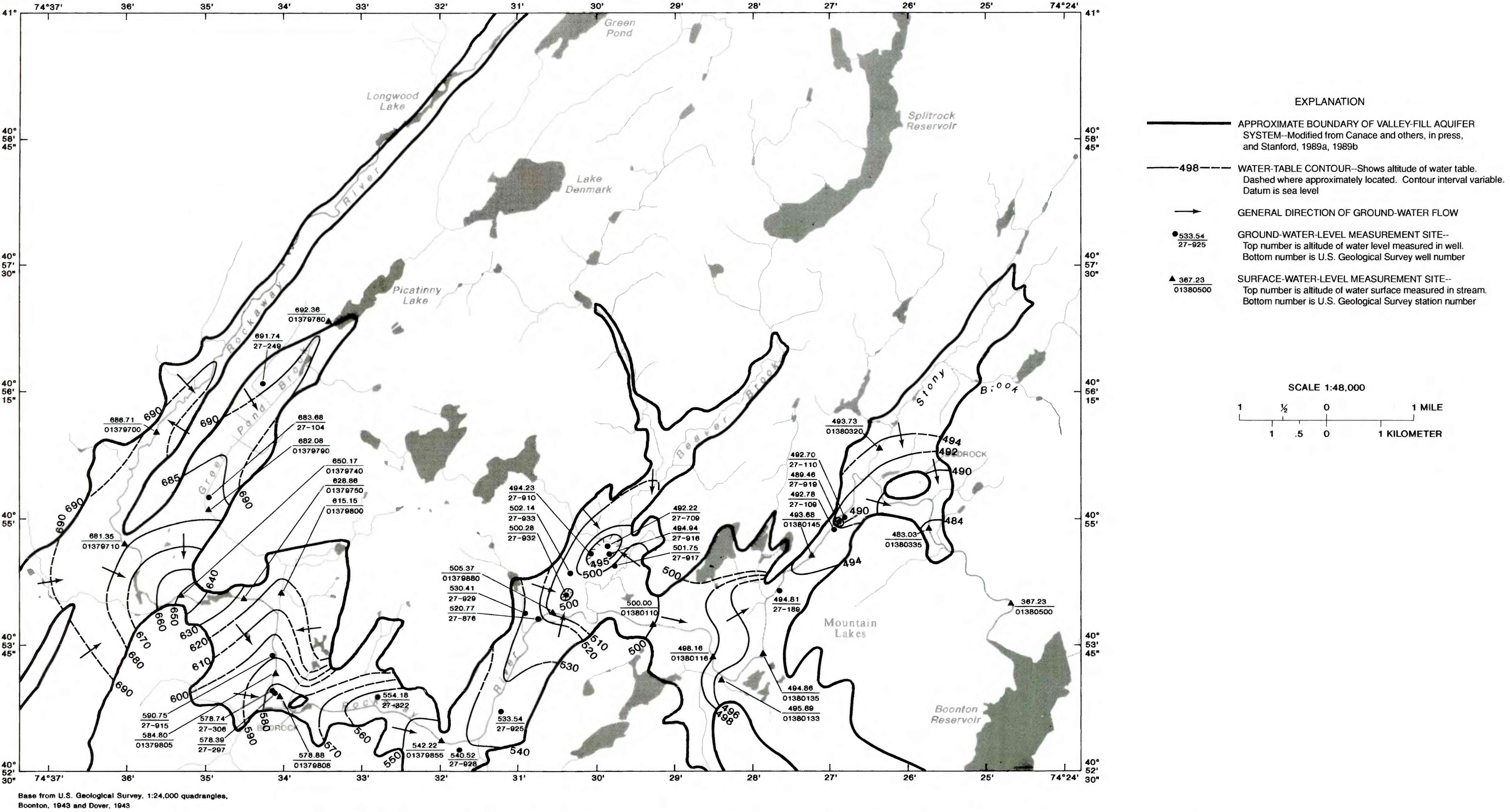
1a. Altitude of water table and general direction of ground-water flow in the unconfined valley-fill aquifer, June-August 1986.
