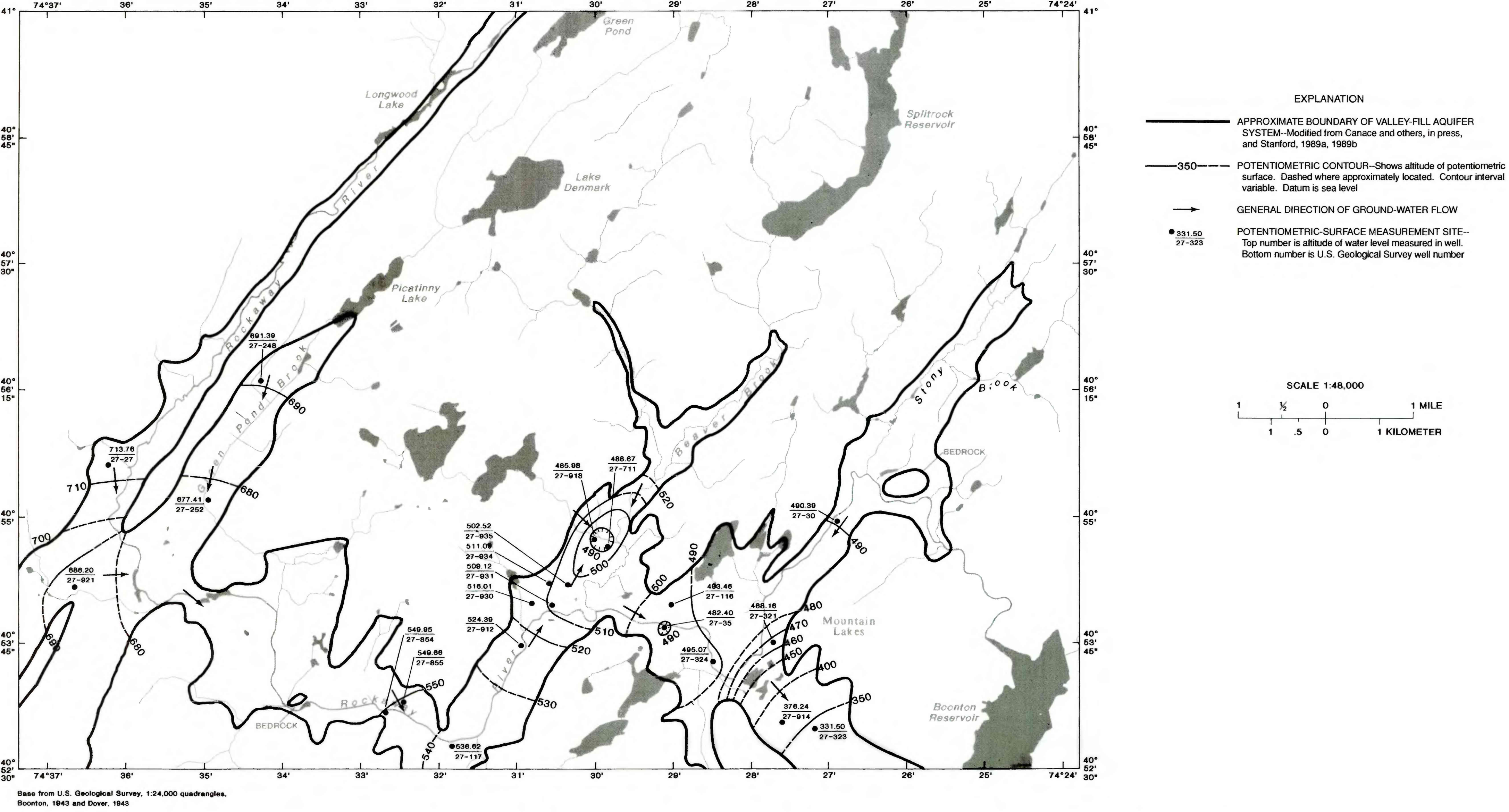
1b. Altitude of potentiometric surface and general direction of ground-water flow in the confined valley-fill aquifer, June-August 1986.
