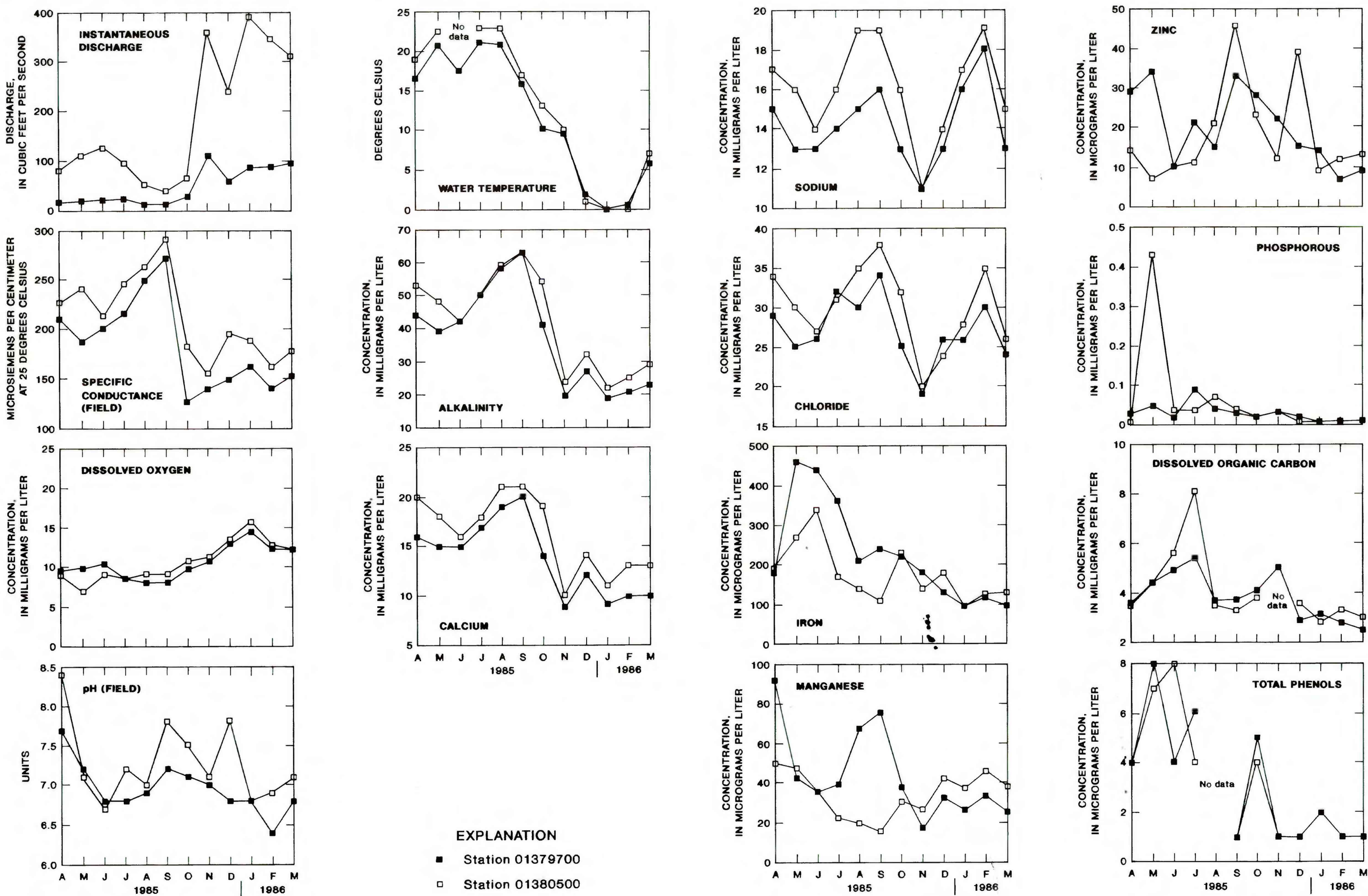
2b. Monthly discharge and water quality at two streamflow-gaging stations on the Rockaway River, April 1985-March 1986.
