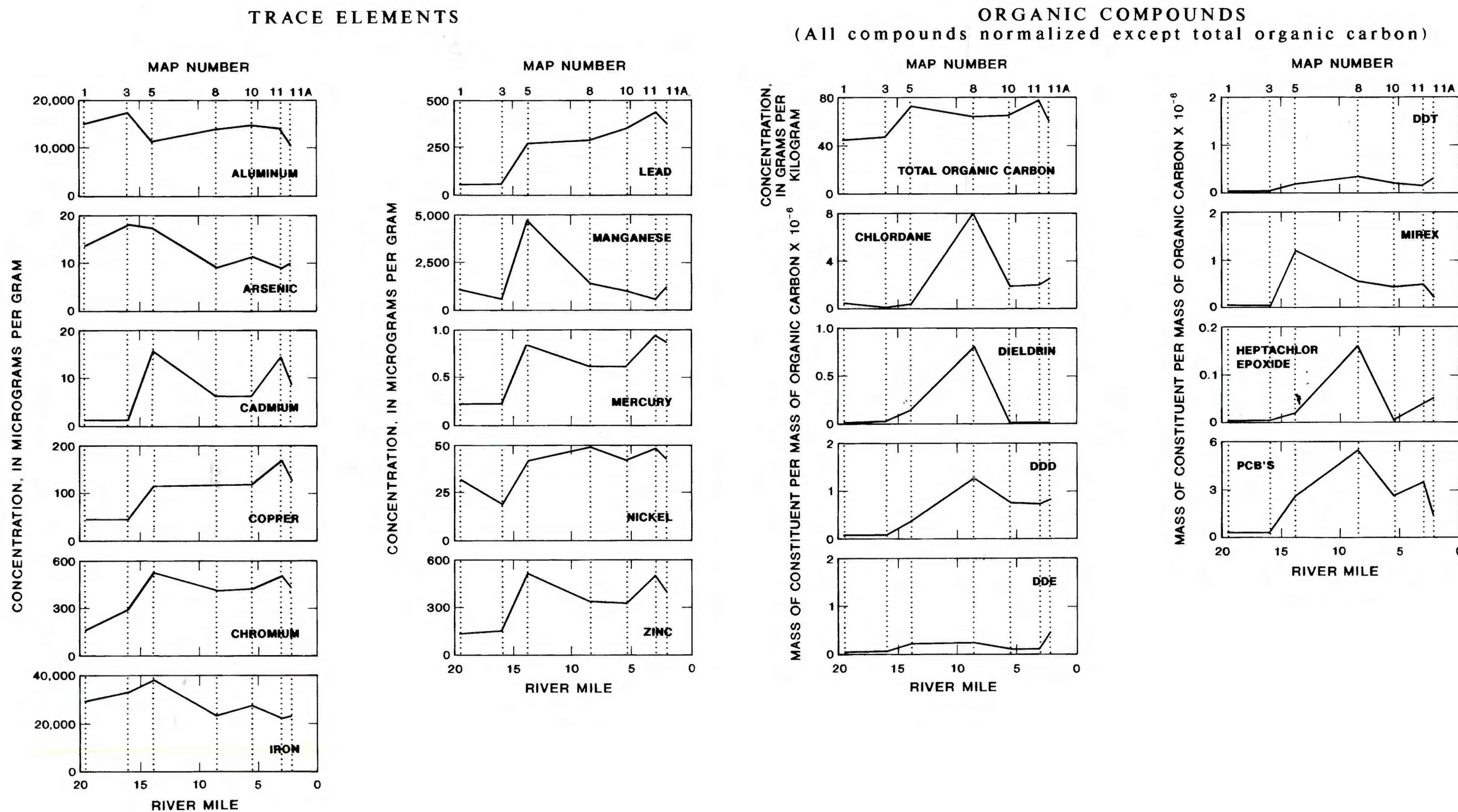
2c. Chemical-quality profiles of streambed material in the Rockaway River, August 14-16, 1985.
