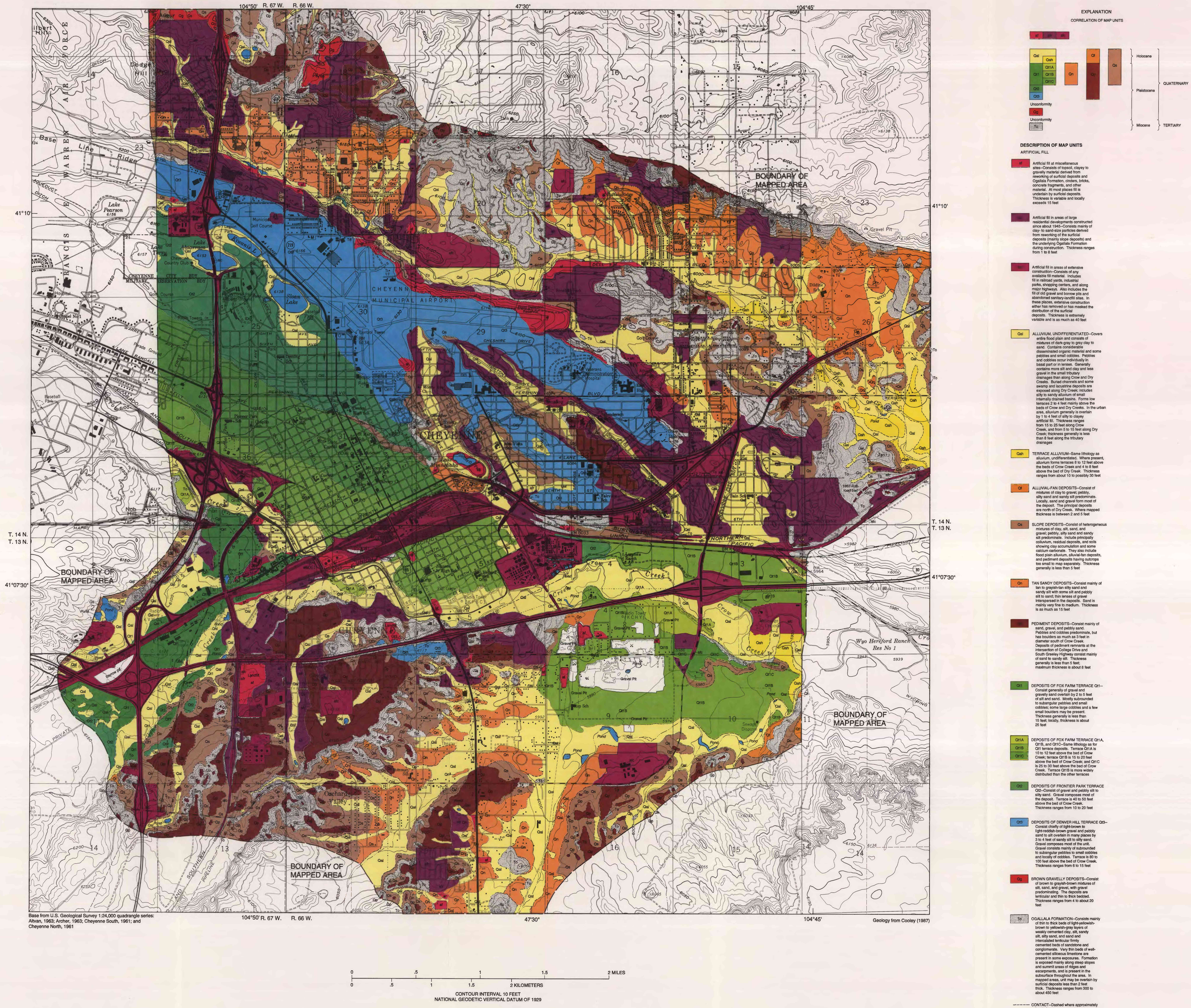
FIGURE 5.—Surficial geology of the Cheyenne urban area.
