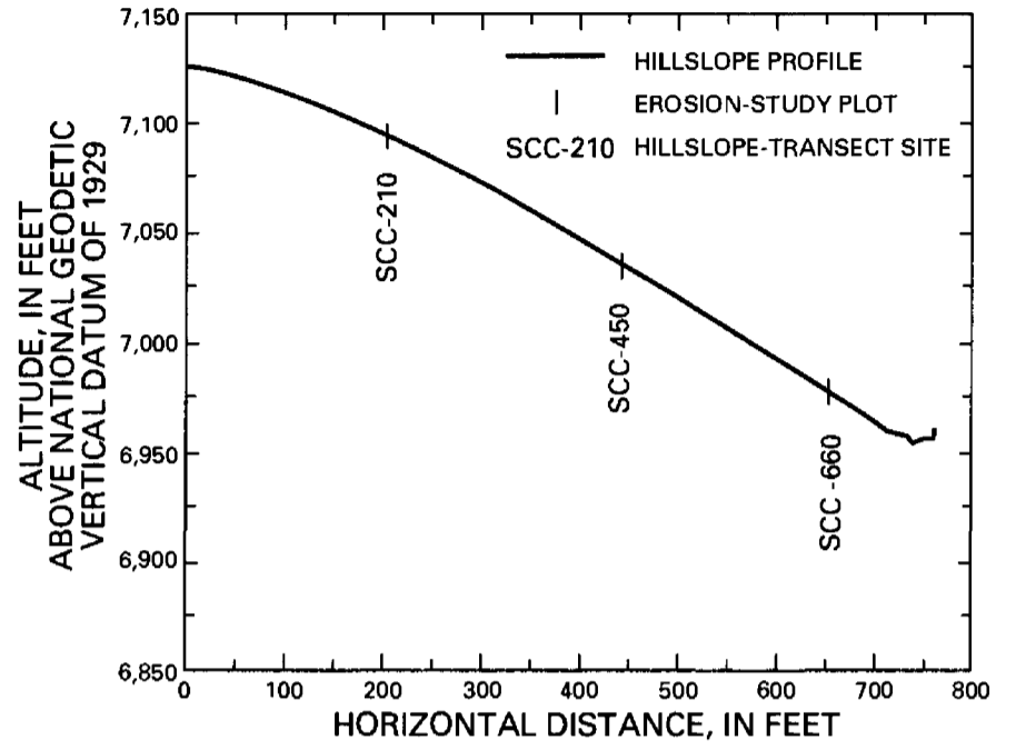
Figure 6. Longitudinal profile of hillslope transect SCC.
