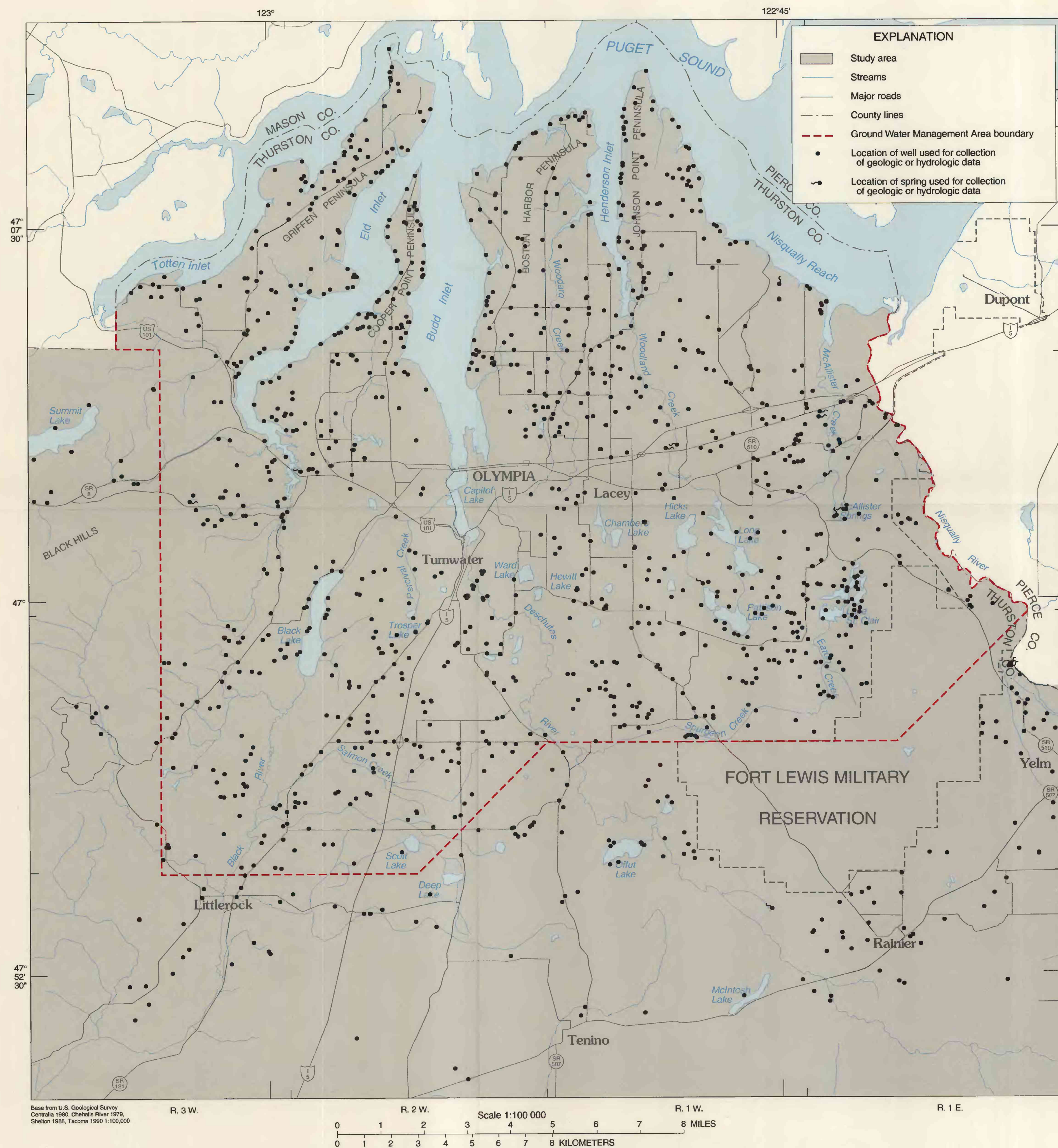
a. Locations of Wells and Springs used to collect Geologic and Hydrologic Data
