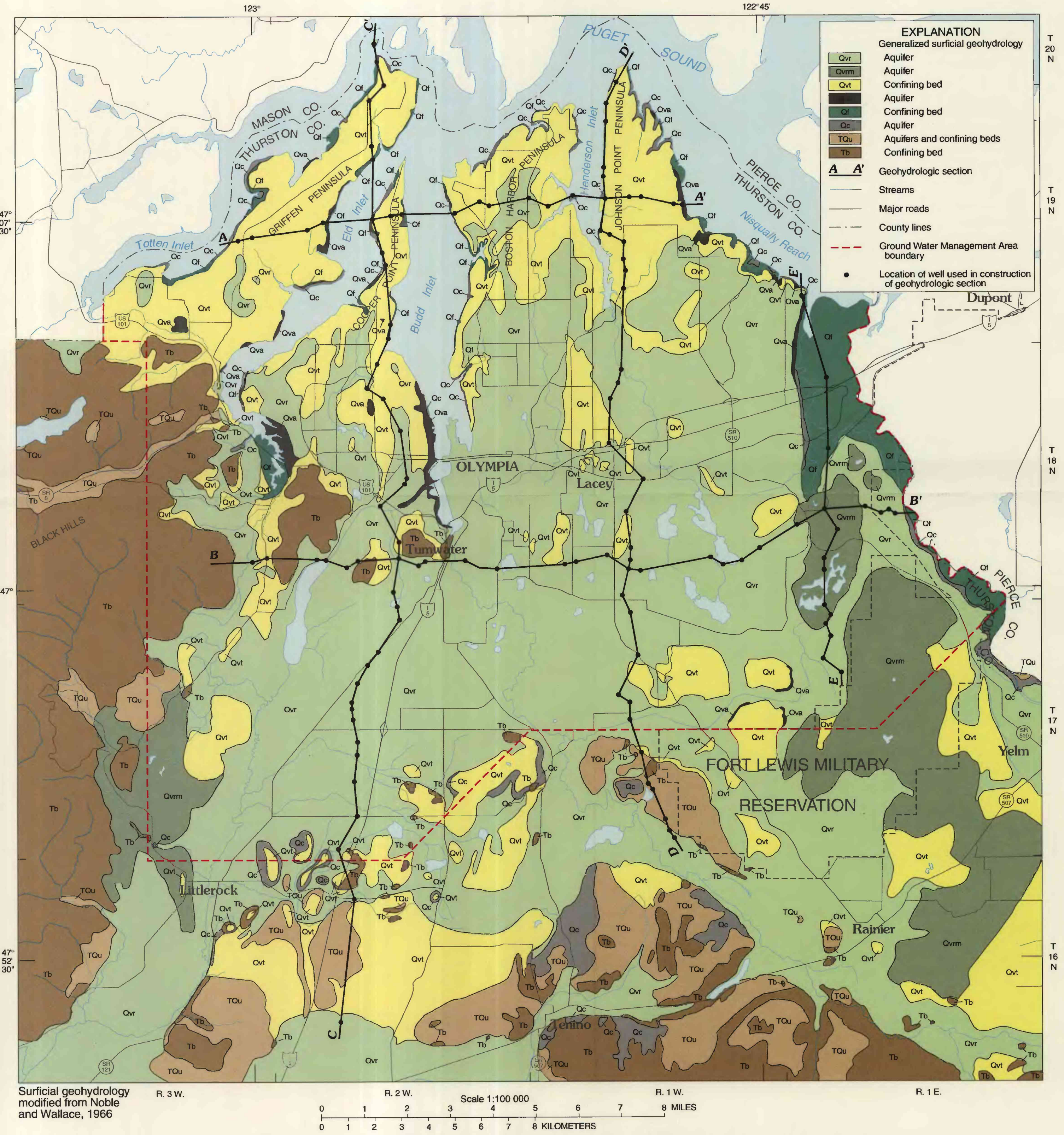
b. Generalized Surficial Geohydrology and Locations of Geohydrologic Sections
