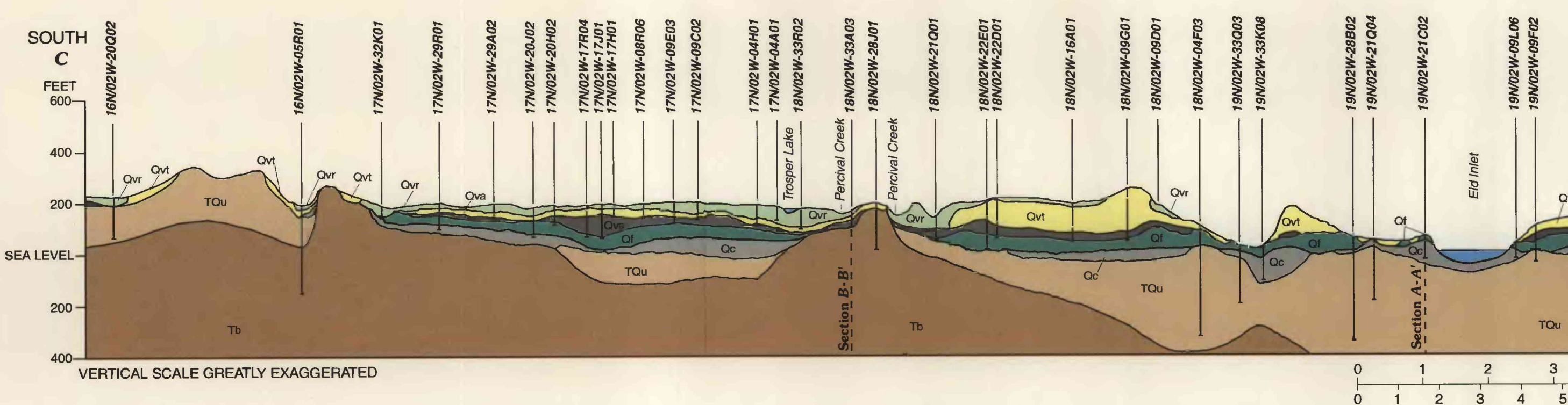
c. Geohydrologic Sections of Northern Thurston County (Total unconsolidated sediment thickness from Jones, 1996)
