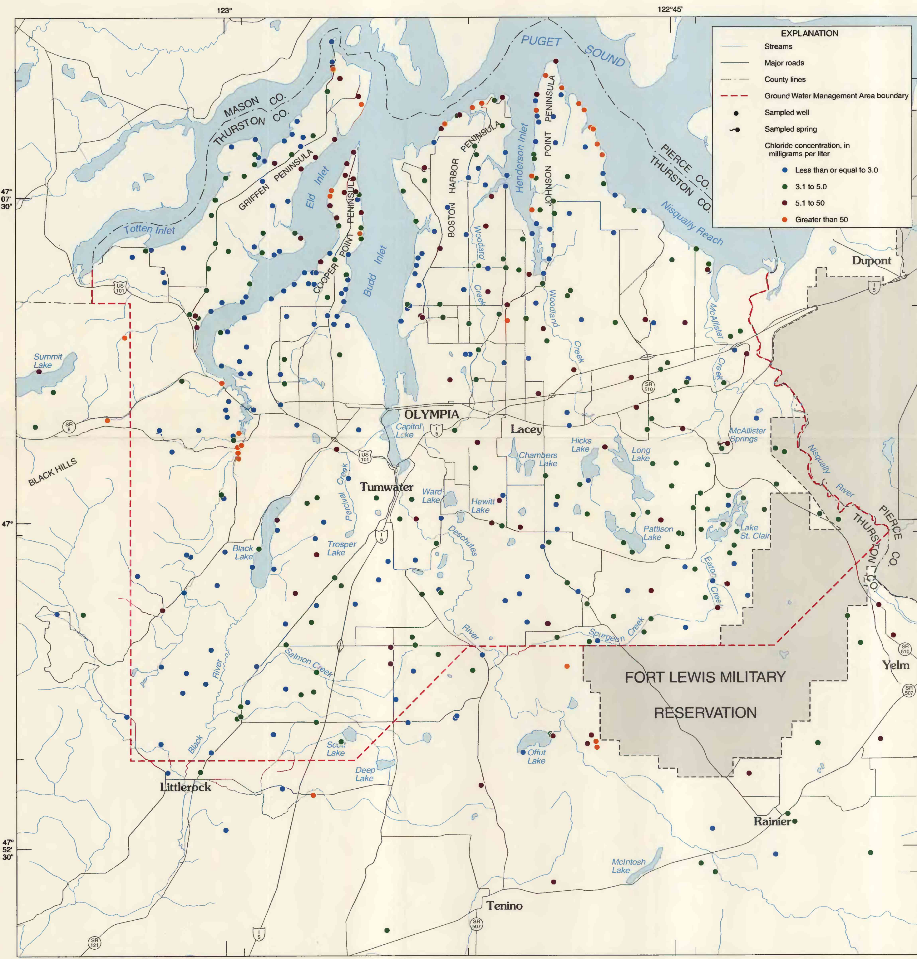
a. Concentrations of Chloride in Ground Water
