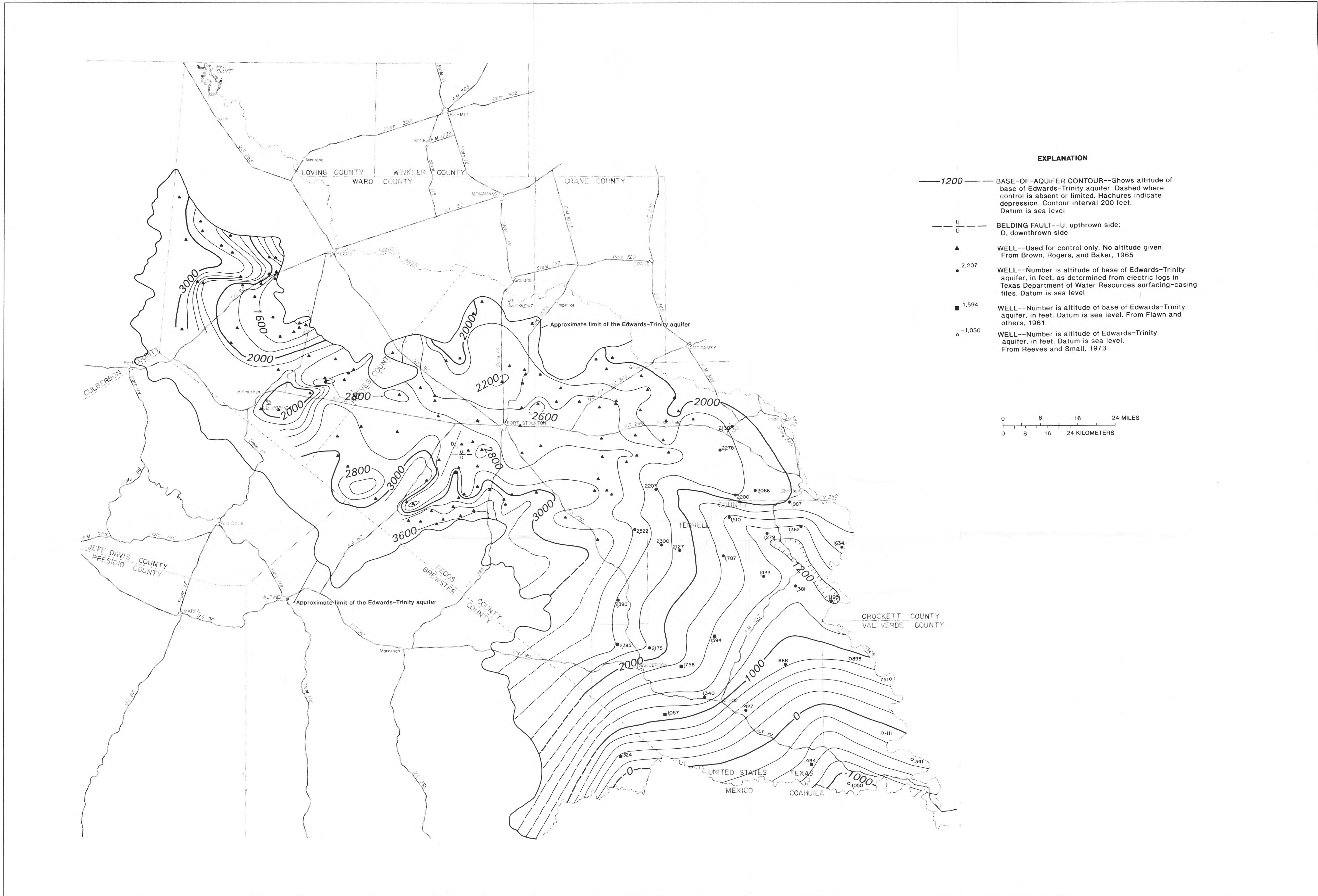
MAP SHOWING APPROXIMATE ALTITUDE OF THE BASE OF THE EDWARDS-TRINITY AQUIFER, TRANS-PECOS REGION, TEXAS. (Modified from Rees and Buckner, 1980, fig.2.)
