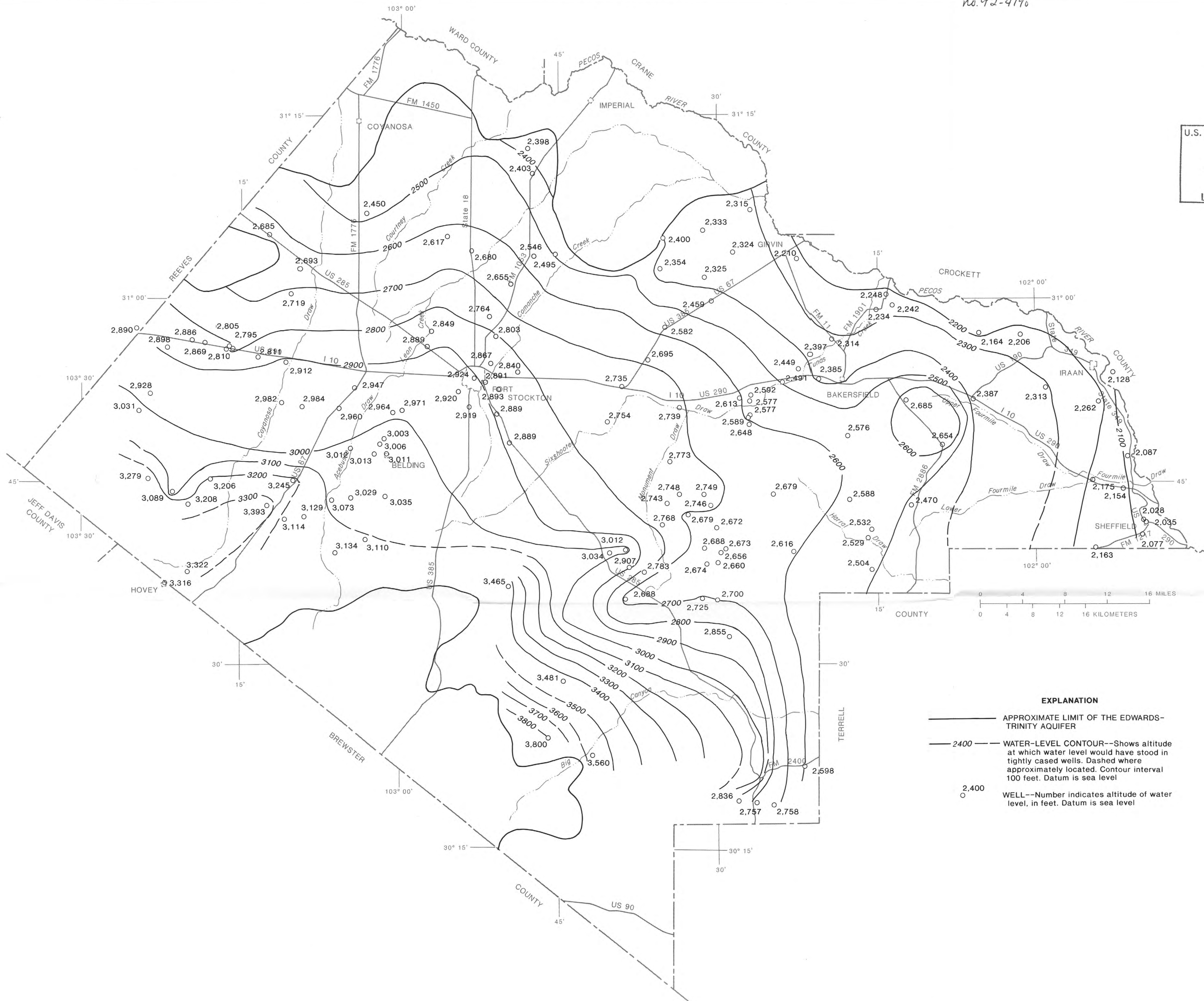
MAP SHOWING 1987 WATER LEVELS IN THE EDWARDS-TRINITY AQUIFER, PECOS COUNTY, TEXAS.
