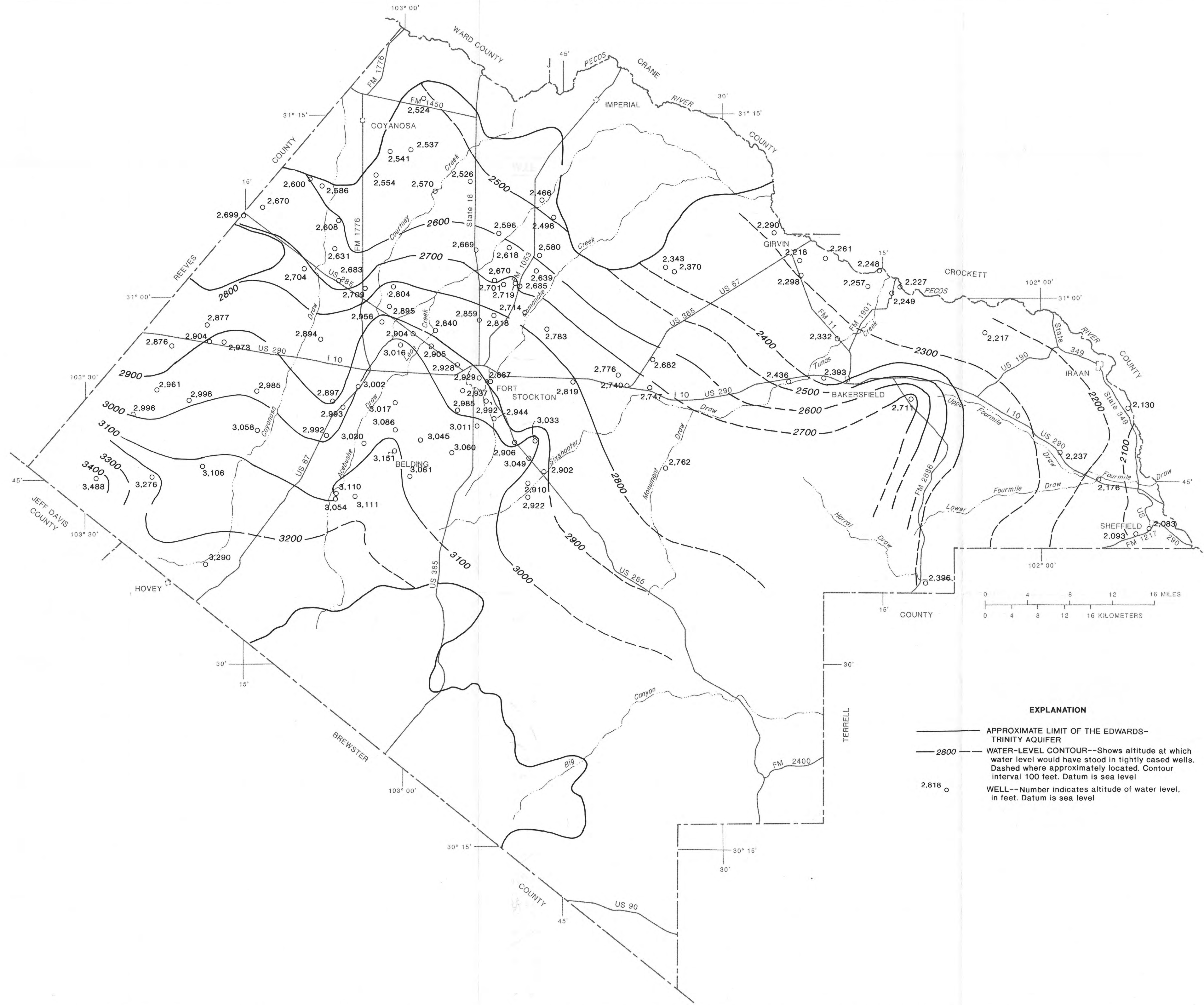
MAP SHOWING HISTORICAL (1940-49) WATER LEVELS IN THE EDWARDS-TRINITY AQUIFER, PECOS COUNTY, TEXAS.
