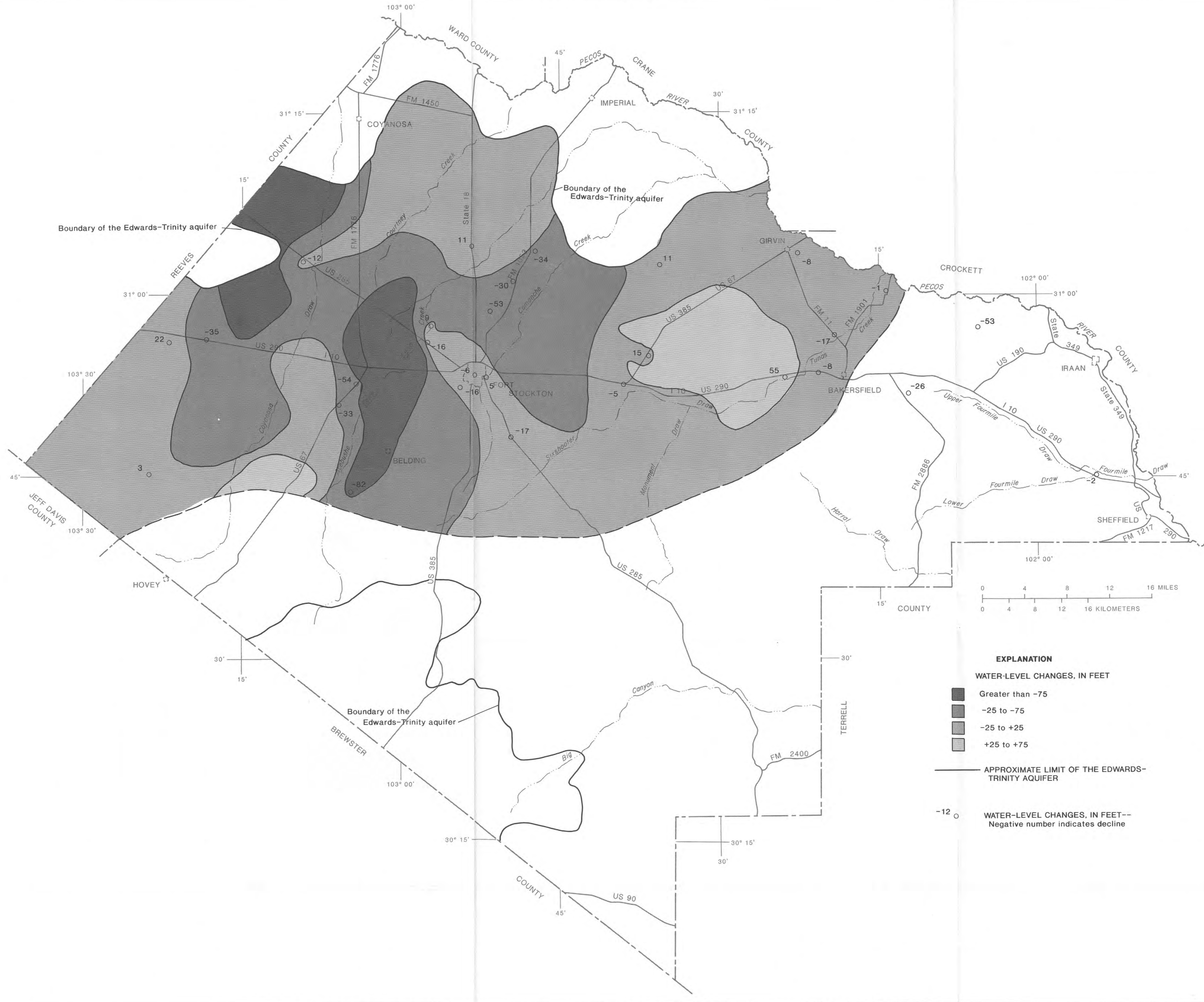
MAP SHOWING CHANGE IN WATER LEVELS IN THE EDWARDS-TRINITY AQUIFER BETWEEN 1940-49 AND 1987, PECOS COUNTY, TEXAS.
