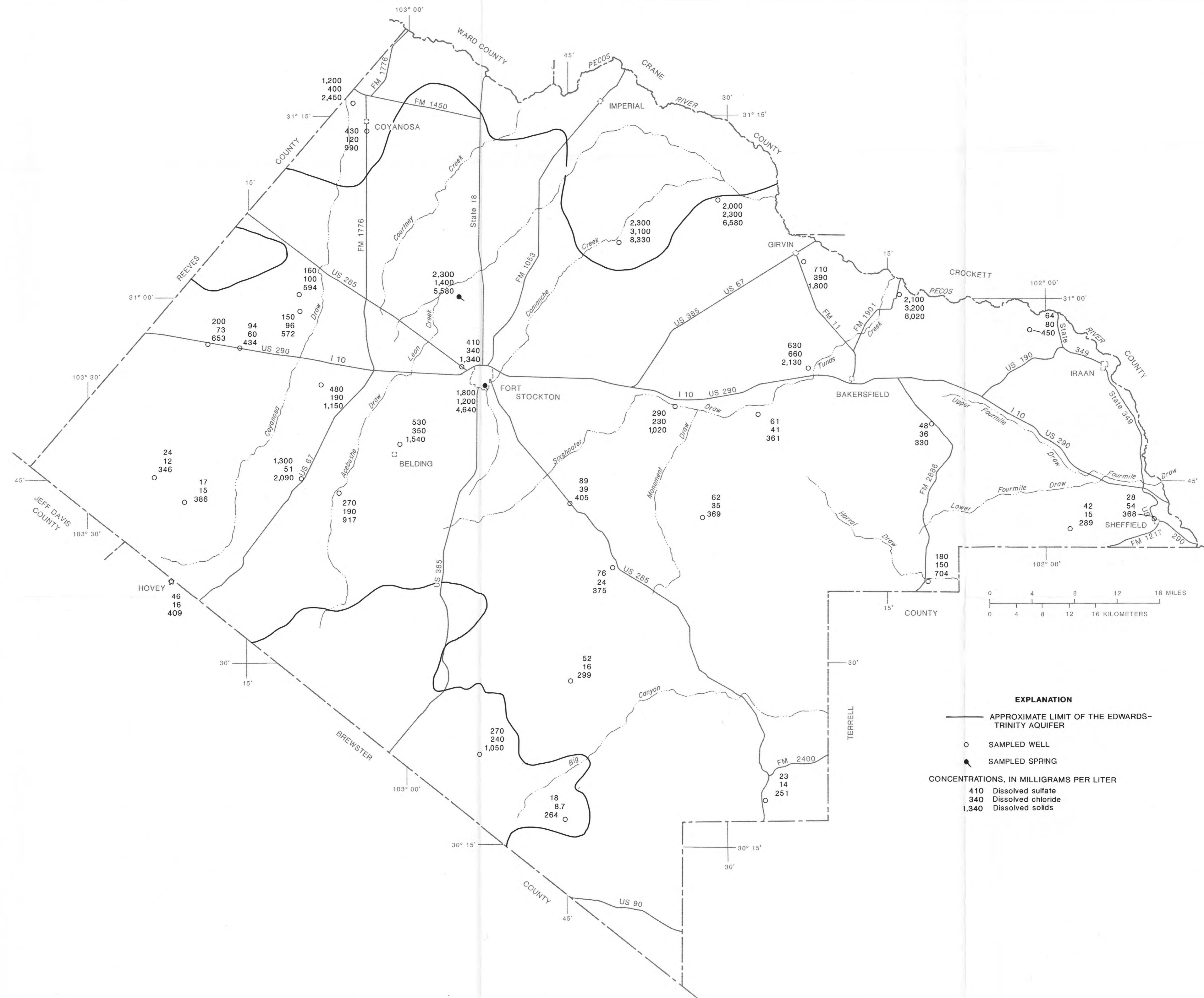
MAP SHOWING DISSOLVED SULFATE, DISSOLVED CHLORIDE, AND DISSOLVED-SOLIDS CONCENTRATIONS IN WATER FROM SELECTED WELLS AND SPRINGS, 1987, PECOS COUNTY, TEXAS.
