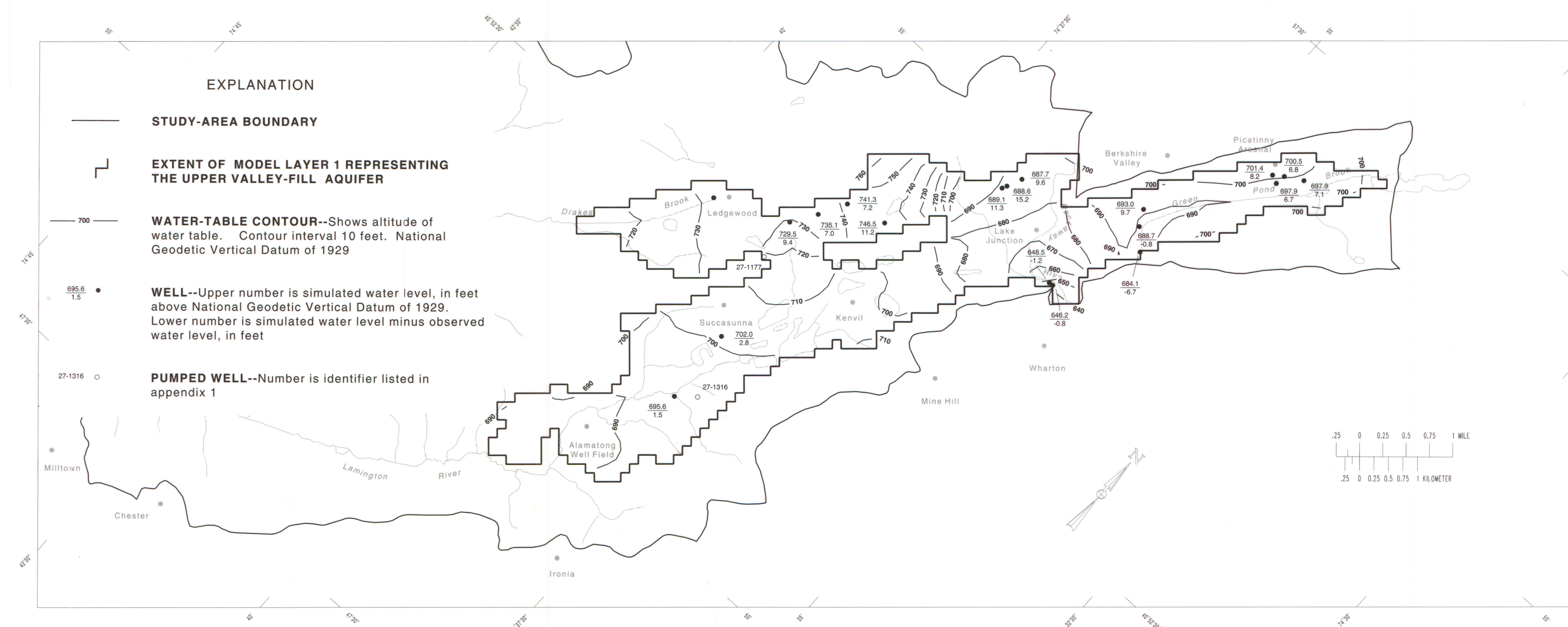
2b. Simulated average water-table surface of the upper valley-fill aquifer, 1988-89, and differences between simulated and observed water levels.
