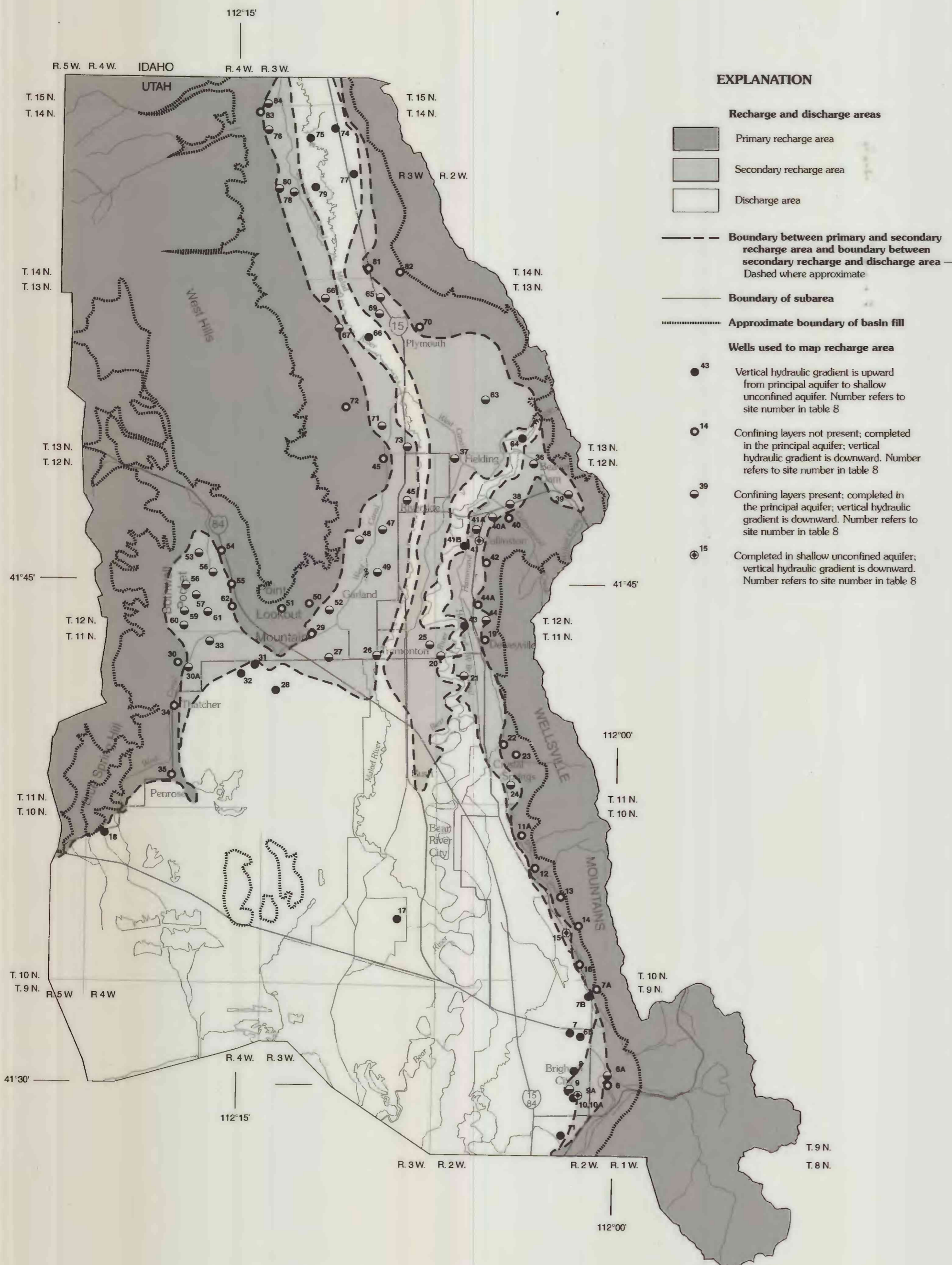
Recharge and discharge areas
