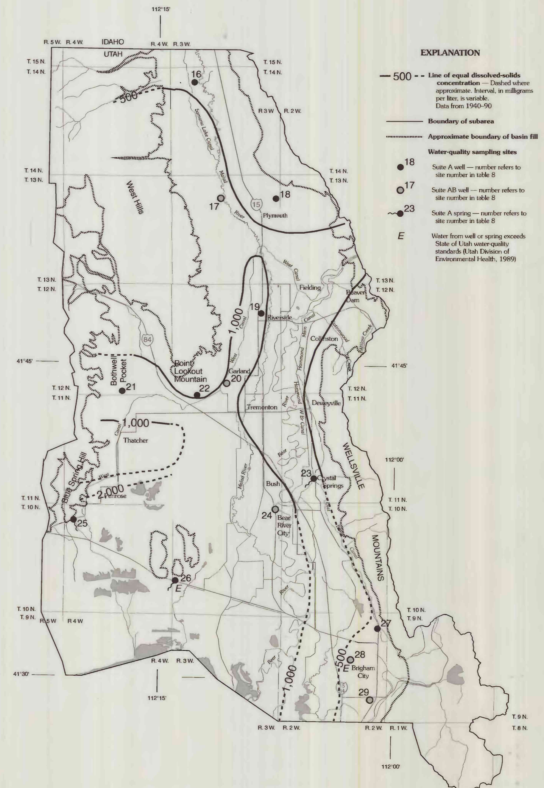
Dissolved-solids concentration and water-quality sampling sites
