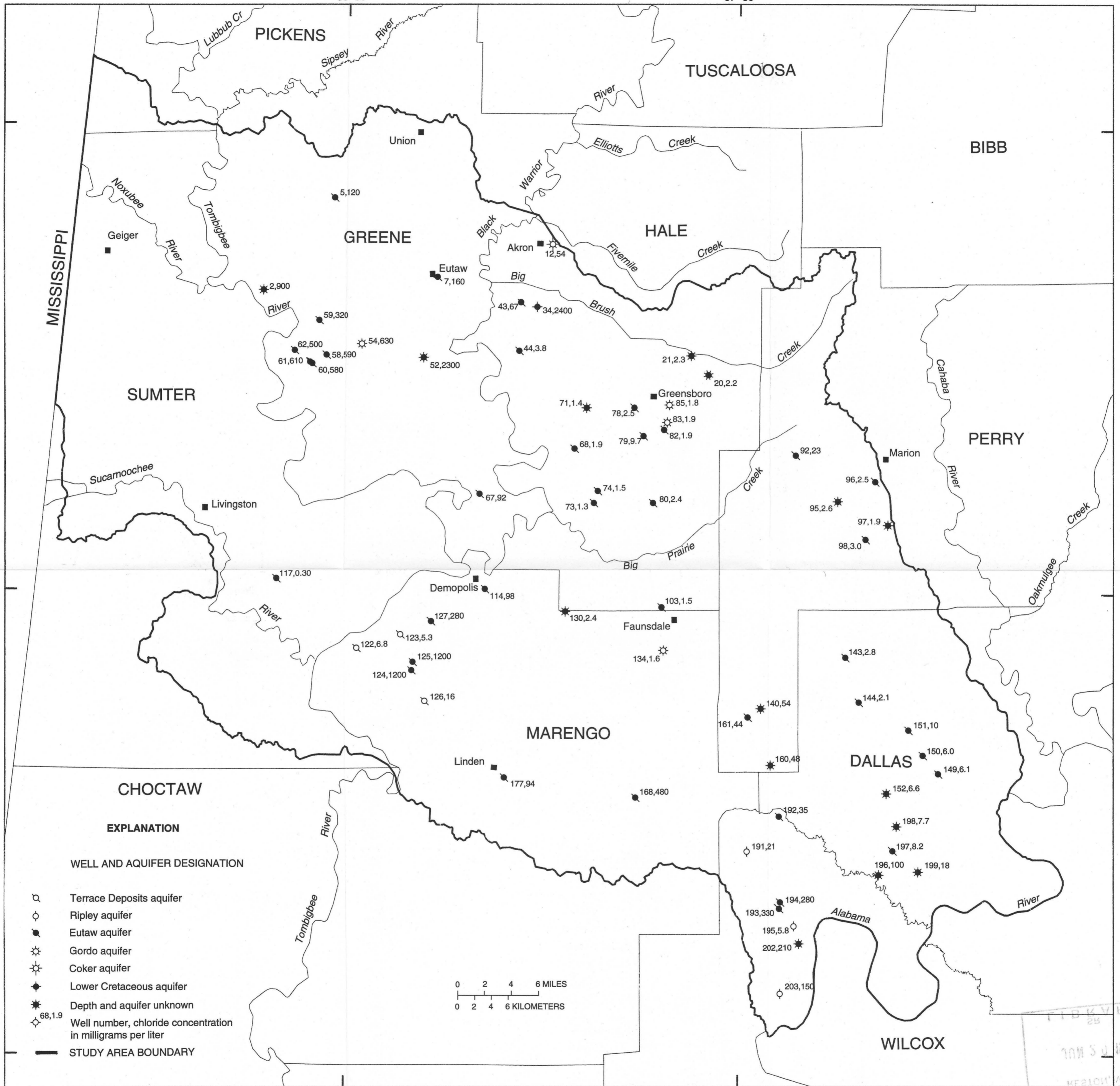
MAP SHOWING DISSOLVED CHLORIDE CONCENTRATIONS IN WATER FROM SELECTED WELLS IN THE BLACK BELT AREA OF WEST-CENTRAL ALABAMA, MARCH 12-21, 1991
