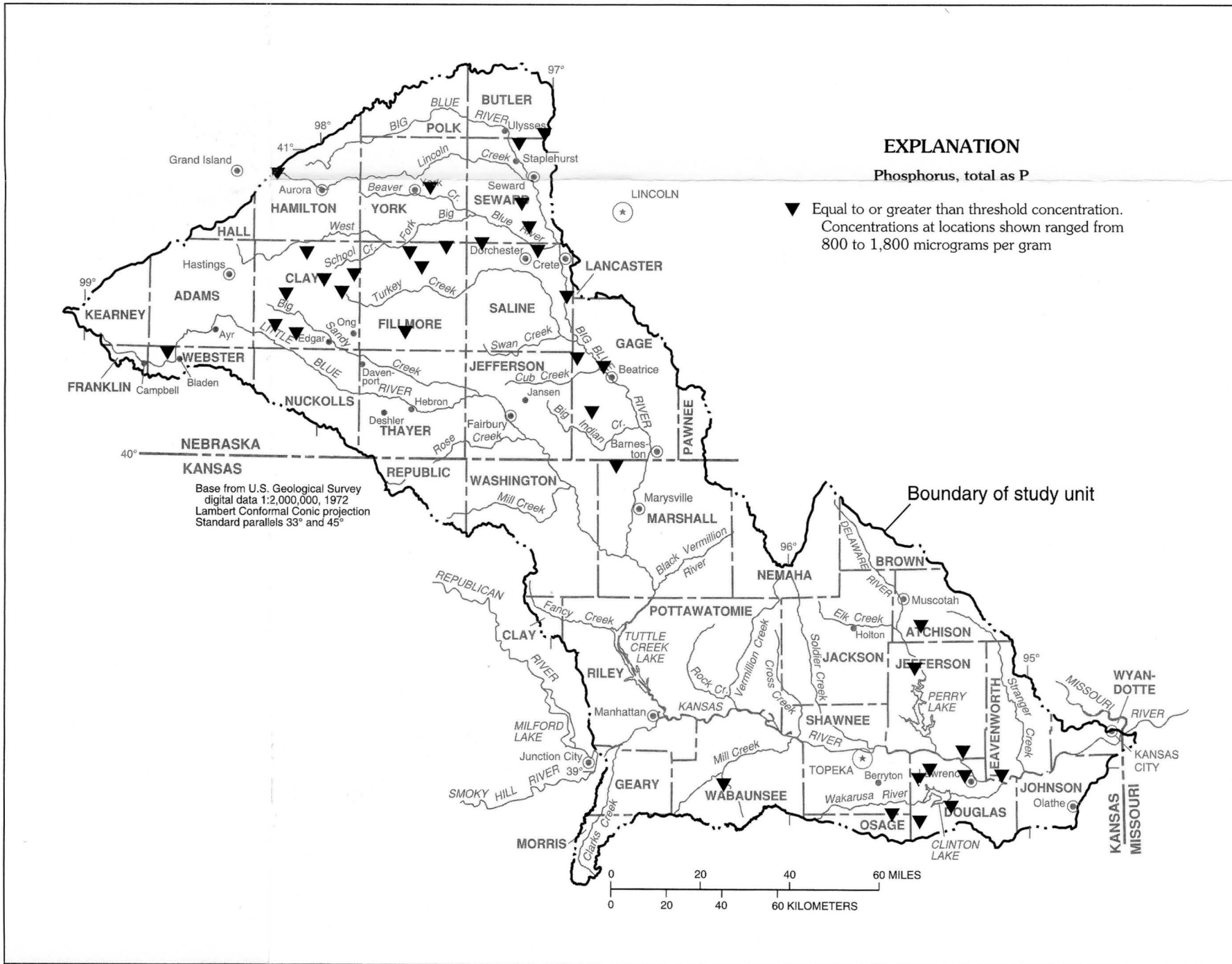
D.--Phosphorous
