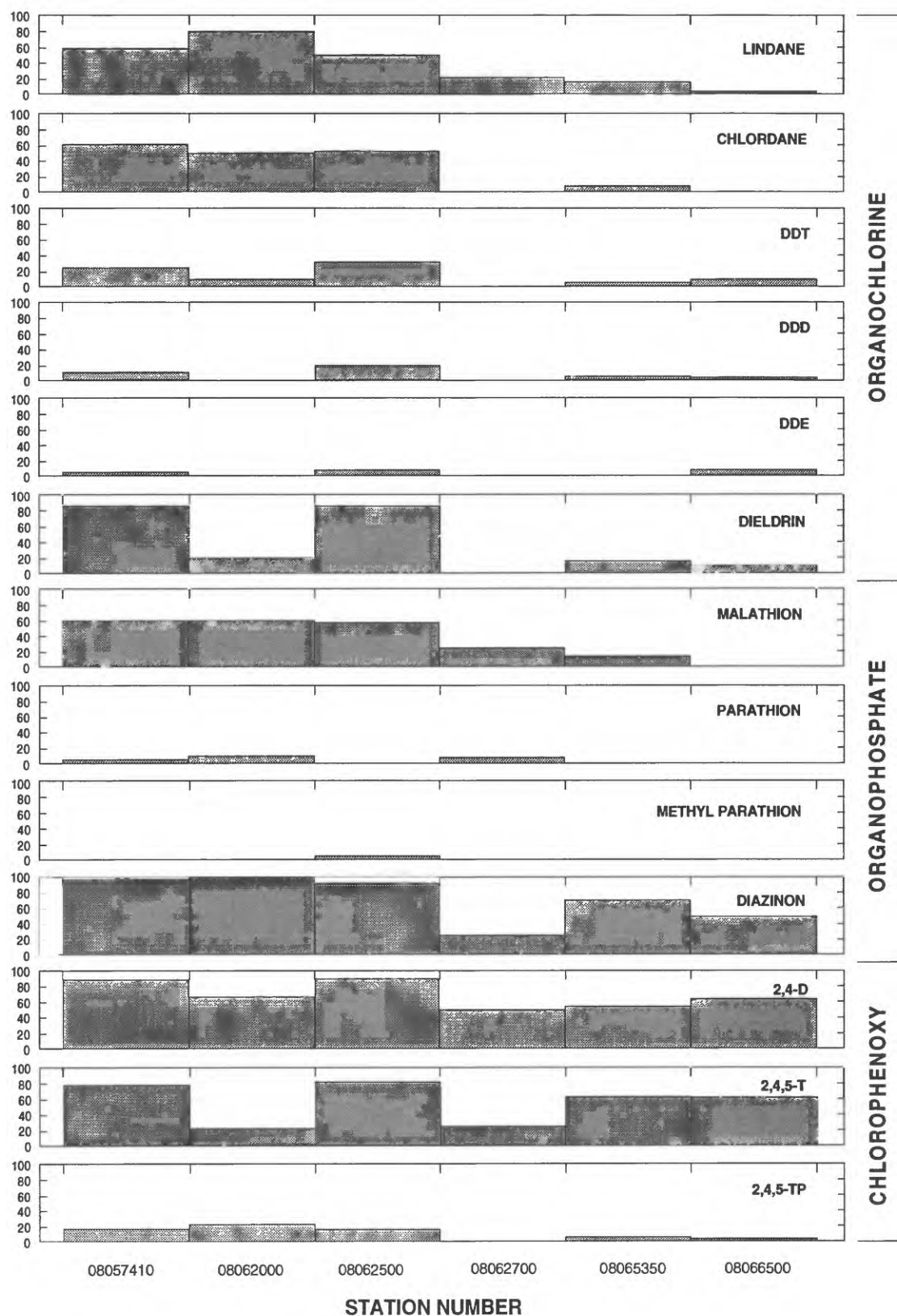
Figure 33. Percent of water samples with pesticides detected at U.S. Geological Survey surface-water-quality stations.
