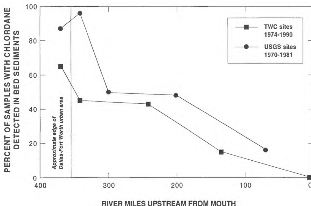
Figure 32. Detections of chlordane in bed sediment at selected U.S. Geological Survey and Texas Water Commission sites during two time periods.
