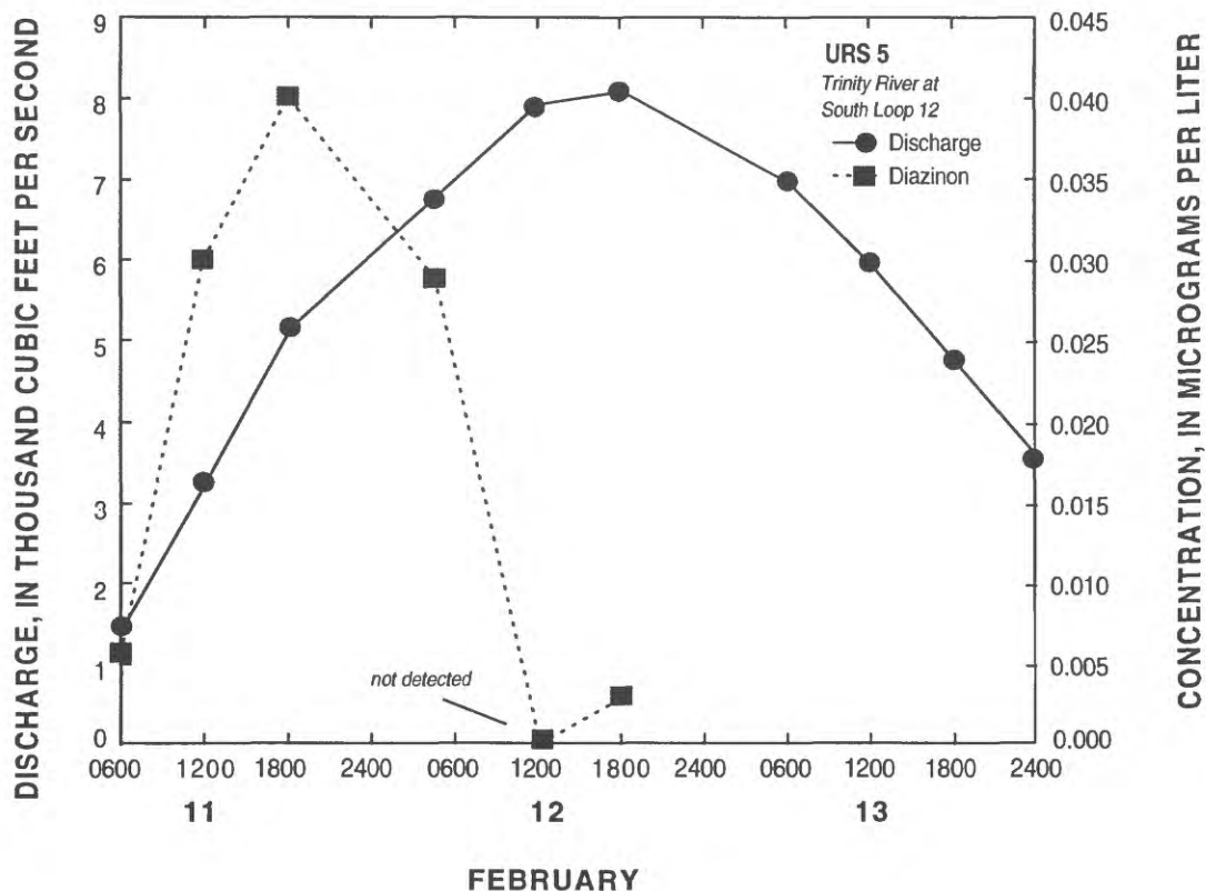
Figure 29. Stream discharge and diazinon concentrations for six samples during 1977 storm, site URS5, Dallas.
