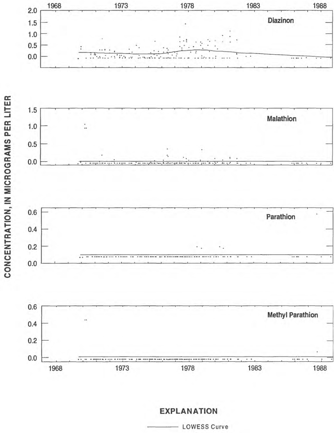
Figure 39. Concentrations of organophosphate pesticides in water at selected U.S. Geological Survey surface-water-quality stations during 1968–89.
