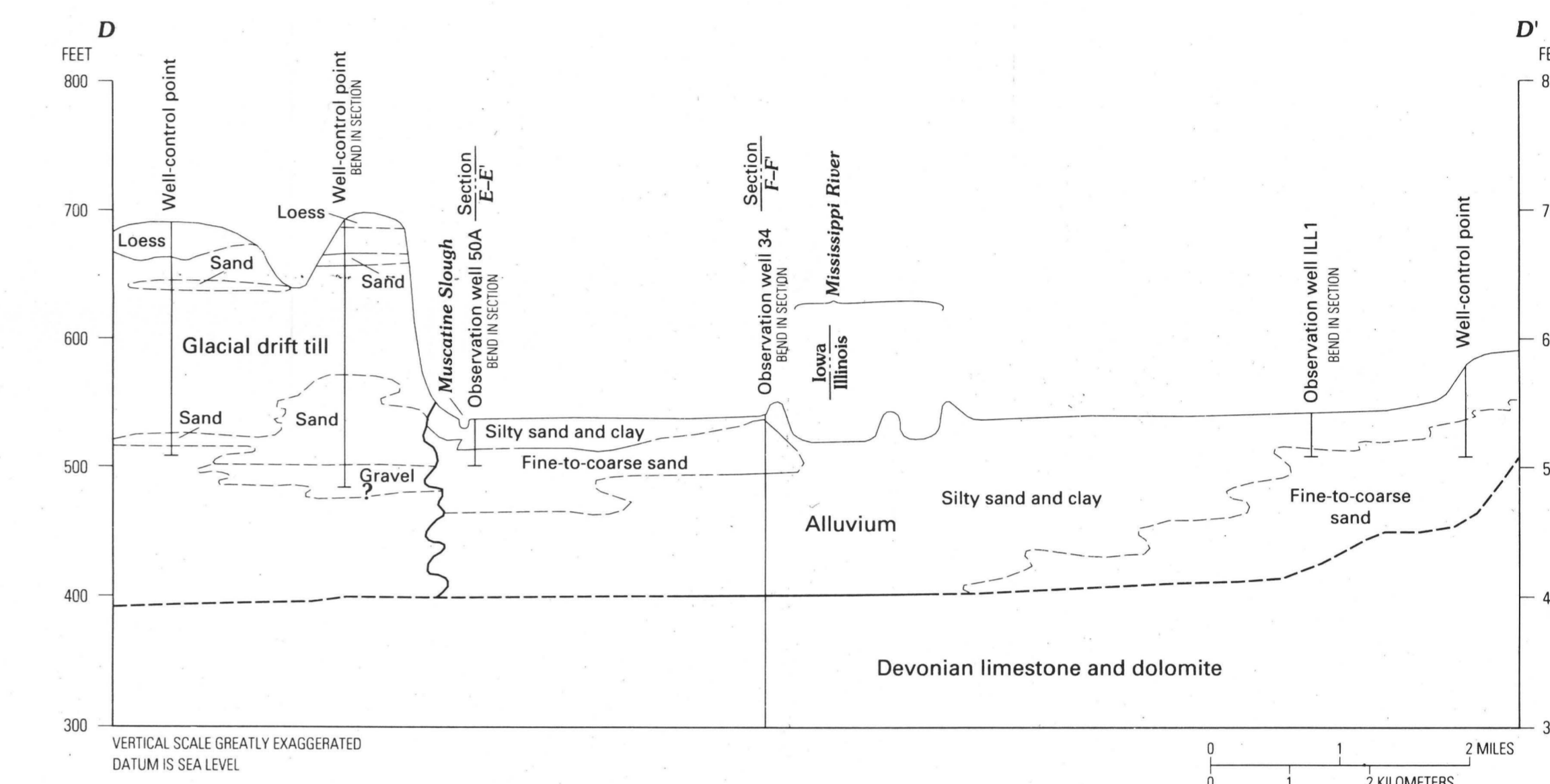
Geologic section D-D'
