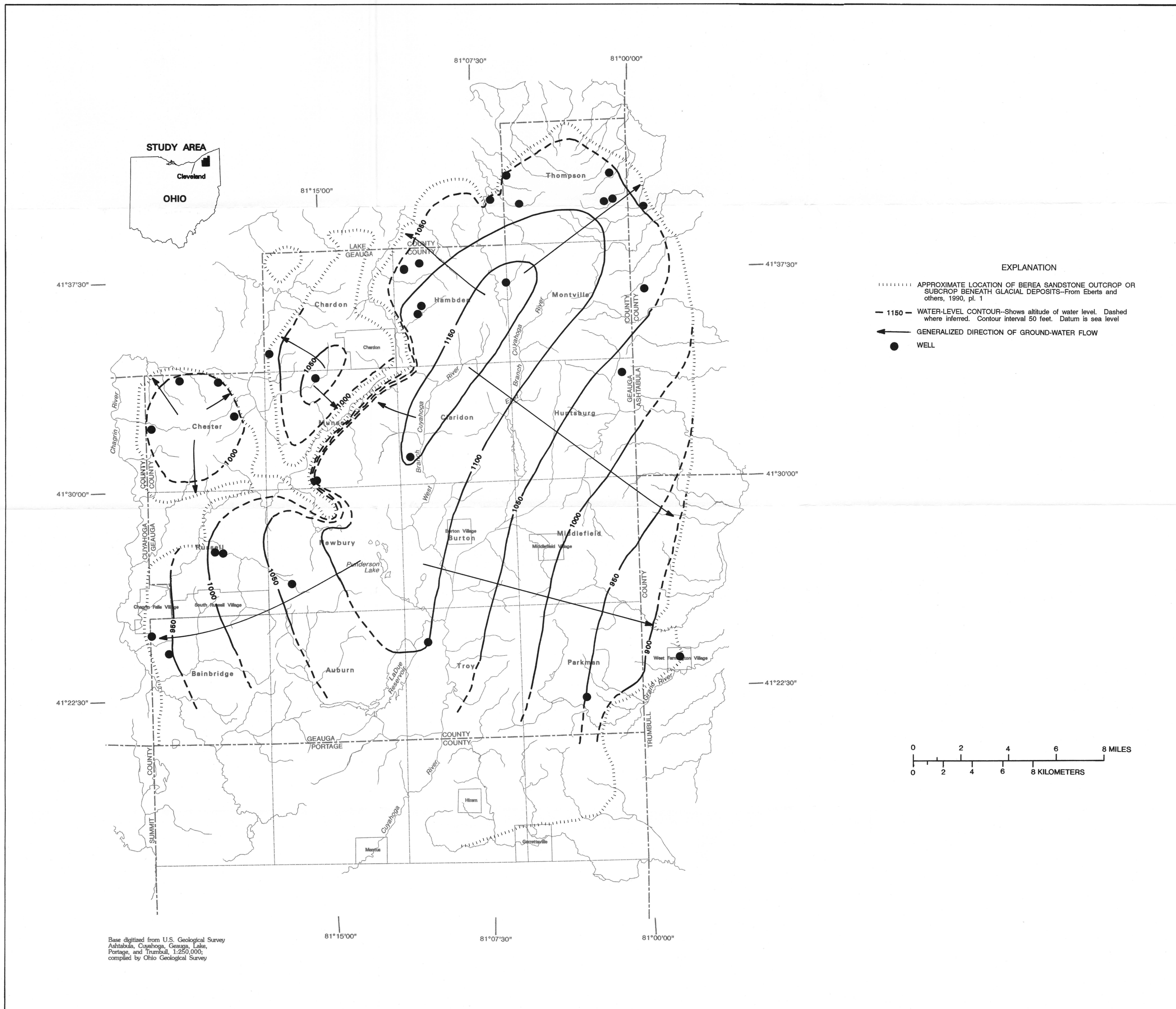
GROUND-WATER LEVELS AND DIRECTION OF FLOW IN THE BEREA SANDSTONE, GEAUGA COUNTY, OHIO, SEPTEMBER 6-9, 1994
