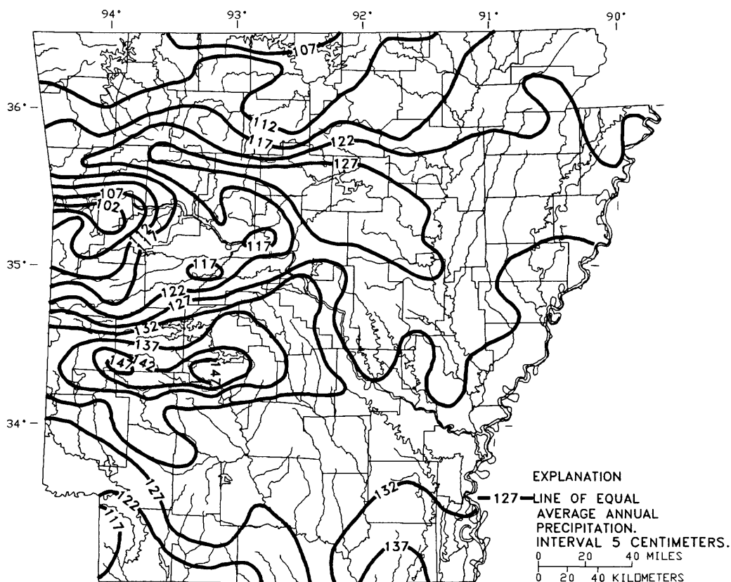
Figure 5. Mean annual precipitation for Arkansas for the base period 1951-80 (from Freiwald, 1985).
