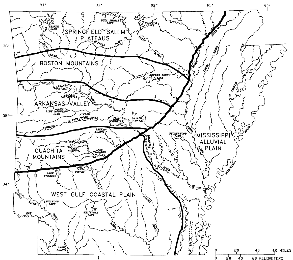
Figure 2. Physiographic provinces in Arkansas.
