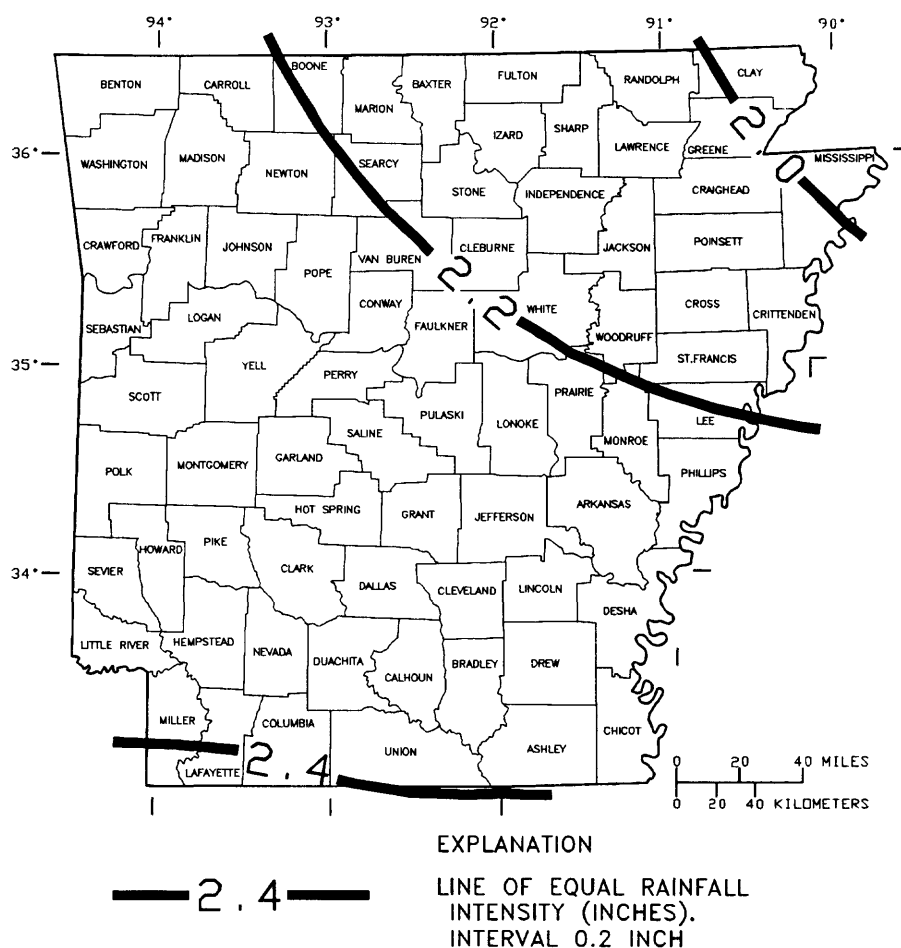
Figure 6. Rainfall intensity for the 2-hour, 2-year occurrence (from Weather Bureau, 1961).
