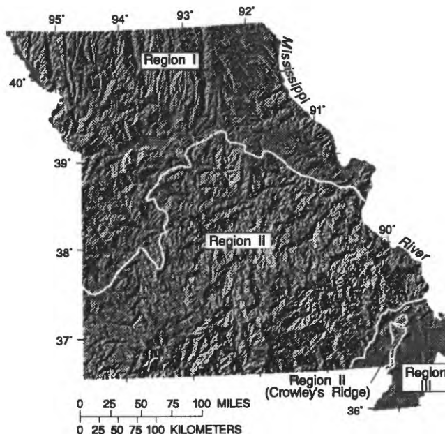
Figure 2. Shaded-relief image of landforms in Missouri and location of hydrologic region boundaries (modified from Thelin and Pike, 1991).
