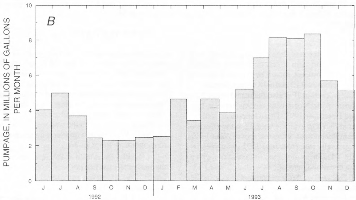
Figure 8. (A) Depth to water at well JF-3 corrected for effects of atmospheric pressure, and (B) combined monthly pumpage at wells J-12 and J-13, Jackass Flats, Nevada, June 1992-December 1993.
