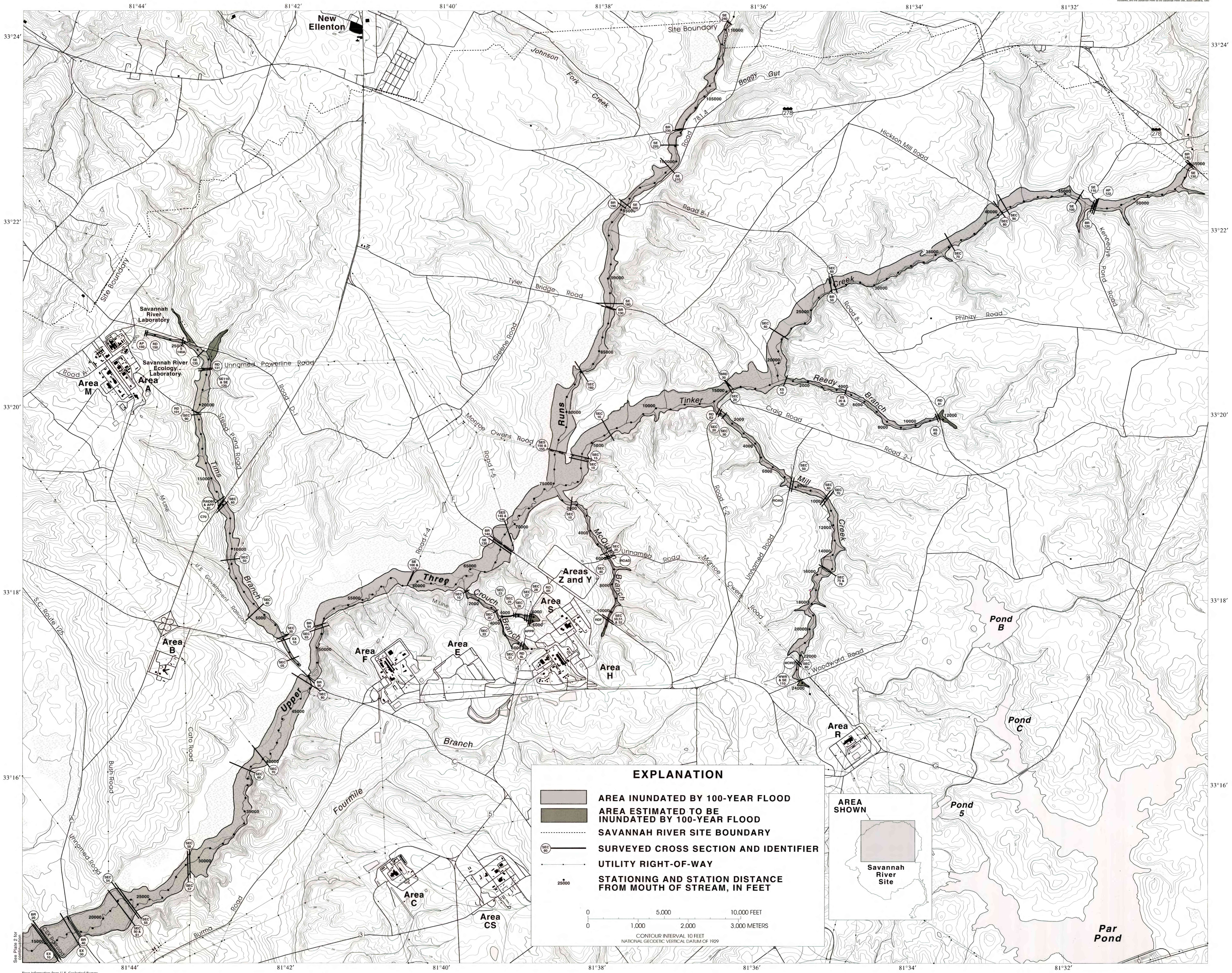
Plate 1. Areal extent of the 100-year flood for Upper Three Runs and selected tributaries at the Savannah River Site, near Aiken, South Carolina.
