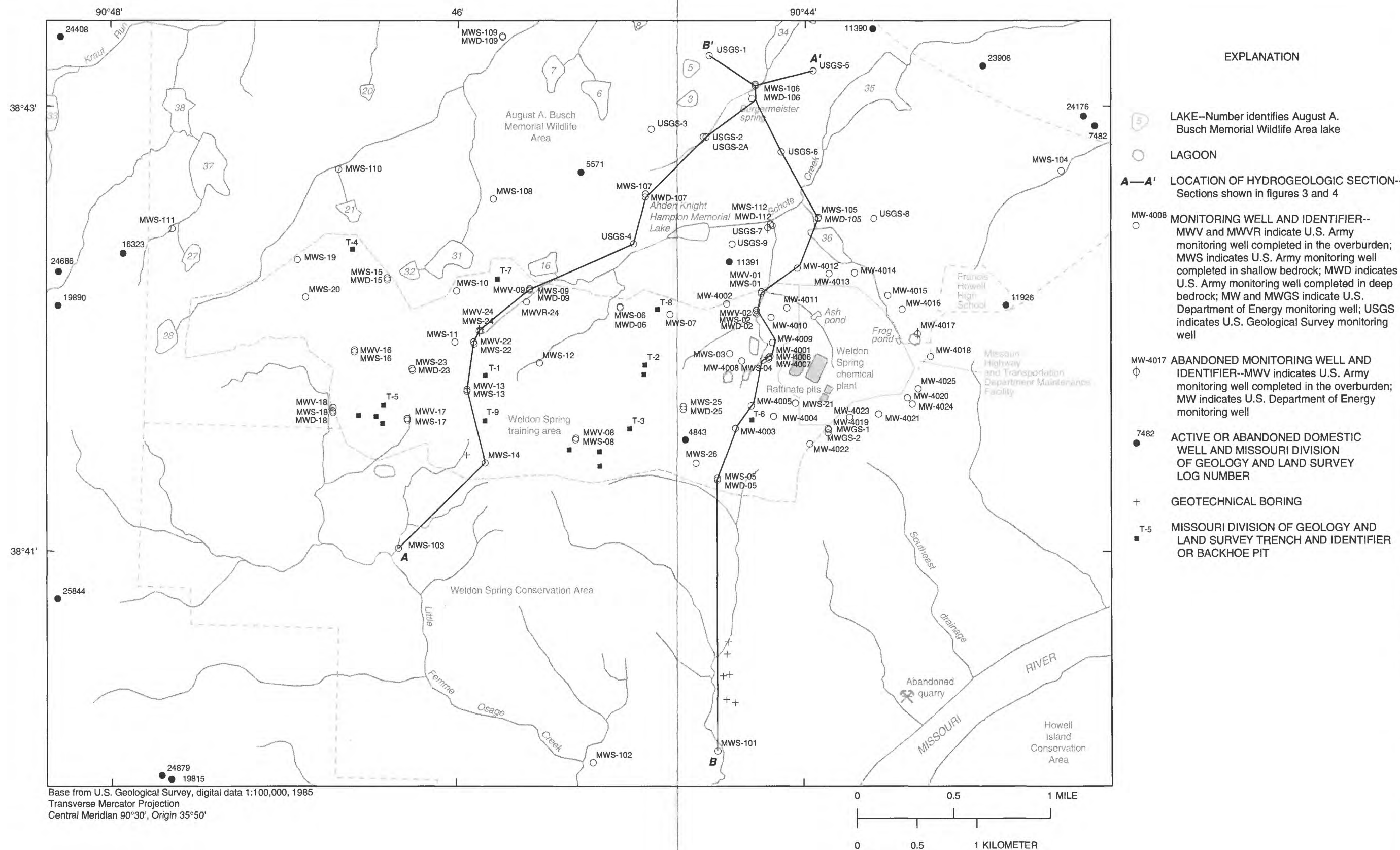
MAP SHOWING LOCATION OF MONITORING WELLS, GEOTECHNICAL BORINGS, DOMESTIC WELLS, AND TRENCHES AT THE WELDON SPRING ORDNANCE WORKS, EXCLUSIVE OF THE WELDON SPRING CHEMICAL PLANT AND THE WELDON SPRING QUARRY, ST. CHARLES COUNTY, MISSOURI
