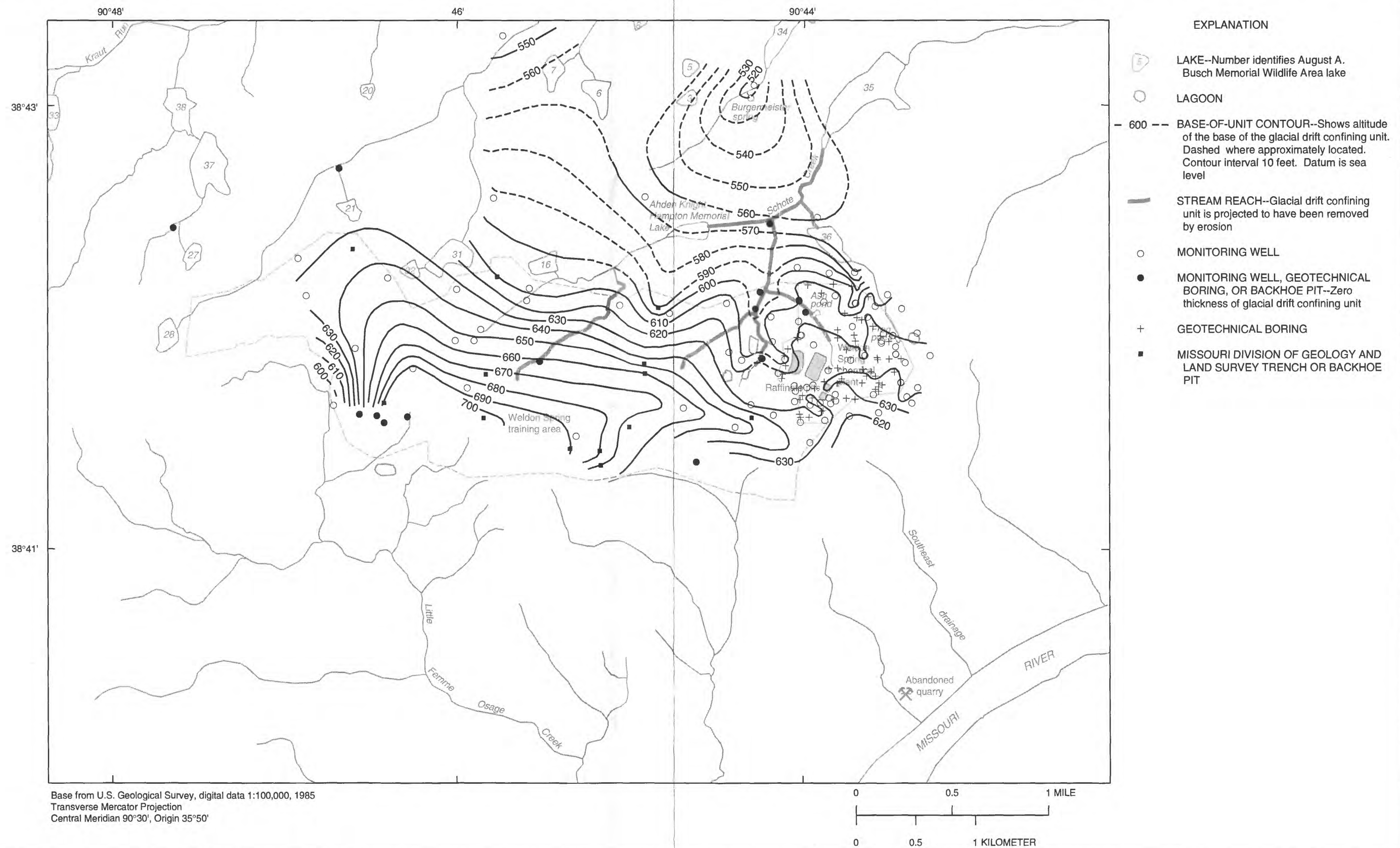
MAP SHOWING ALTITUDE OF THE BASE OF THE GLACIAL DRIFT CONFINING UNIT, WELDON SPRING ORDNANCE WORKS, ST. CHARLES COUNTY, MISSOURI
