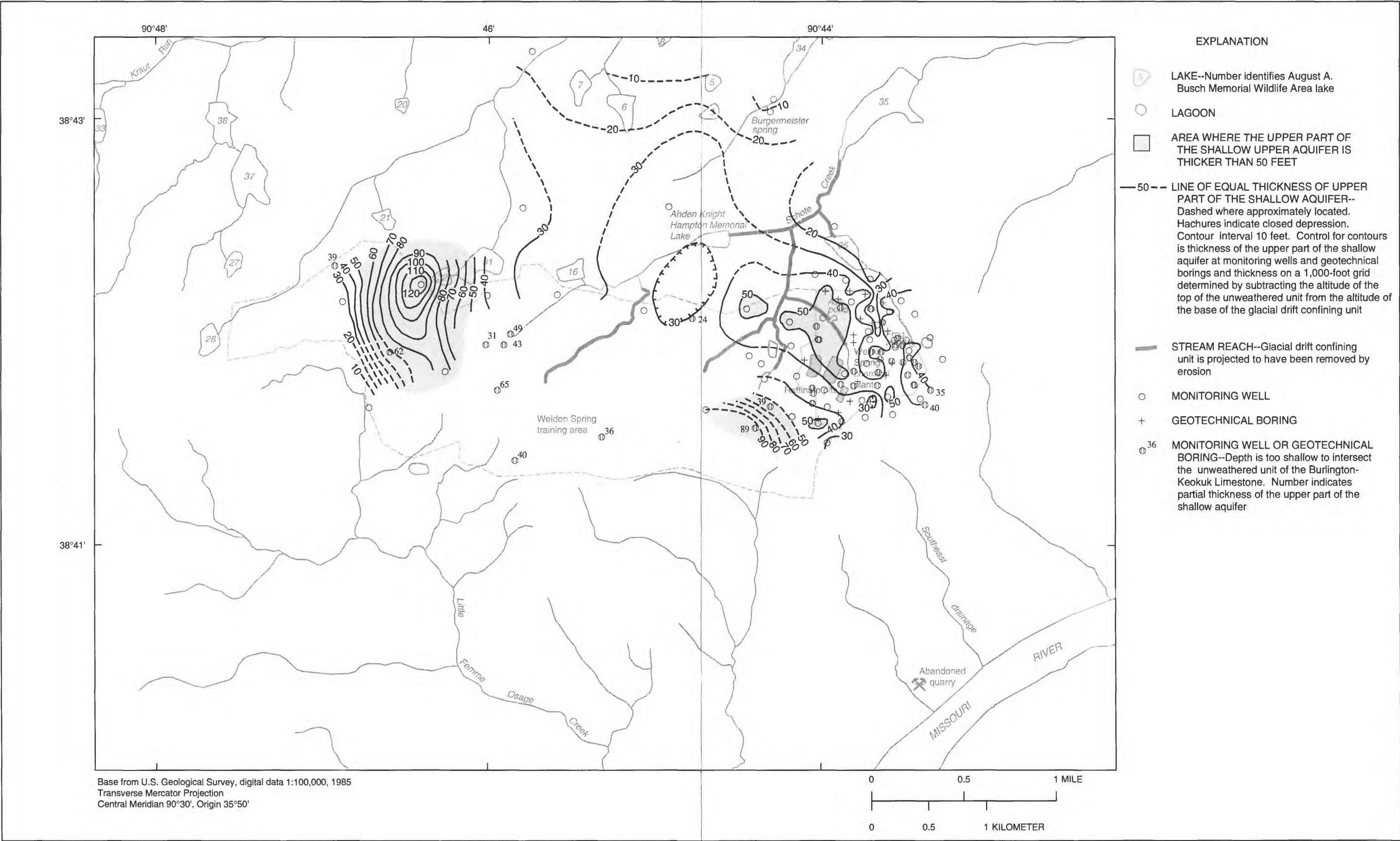
MAP SHOWING THICKNESS OF THE UPPER PART OF THE SHALLOW AQUIFER (BASE OF GLACIAL DRIFT CONFINING UNIT TO TOP OF THE UNWEATHERED UNIT OF THE BURLINGTON-KEOKUK LIMESTONE), WELDON SPRING ORDNANCE WORKS, ST. CHARLES COUNTY, MISSOURI
