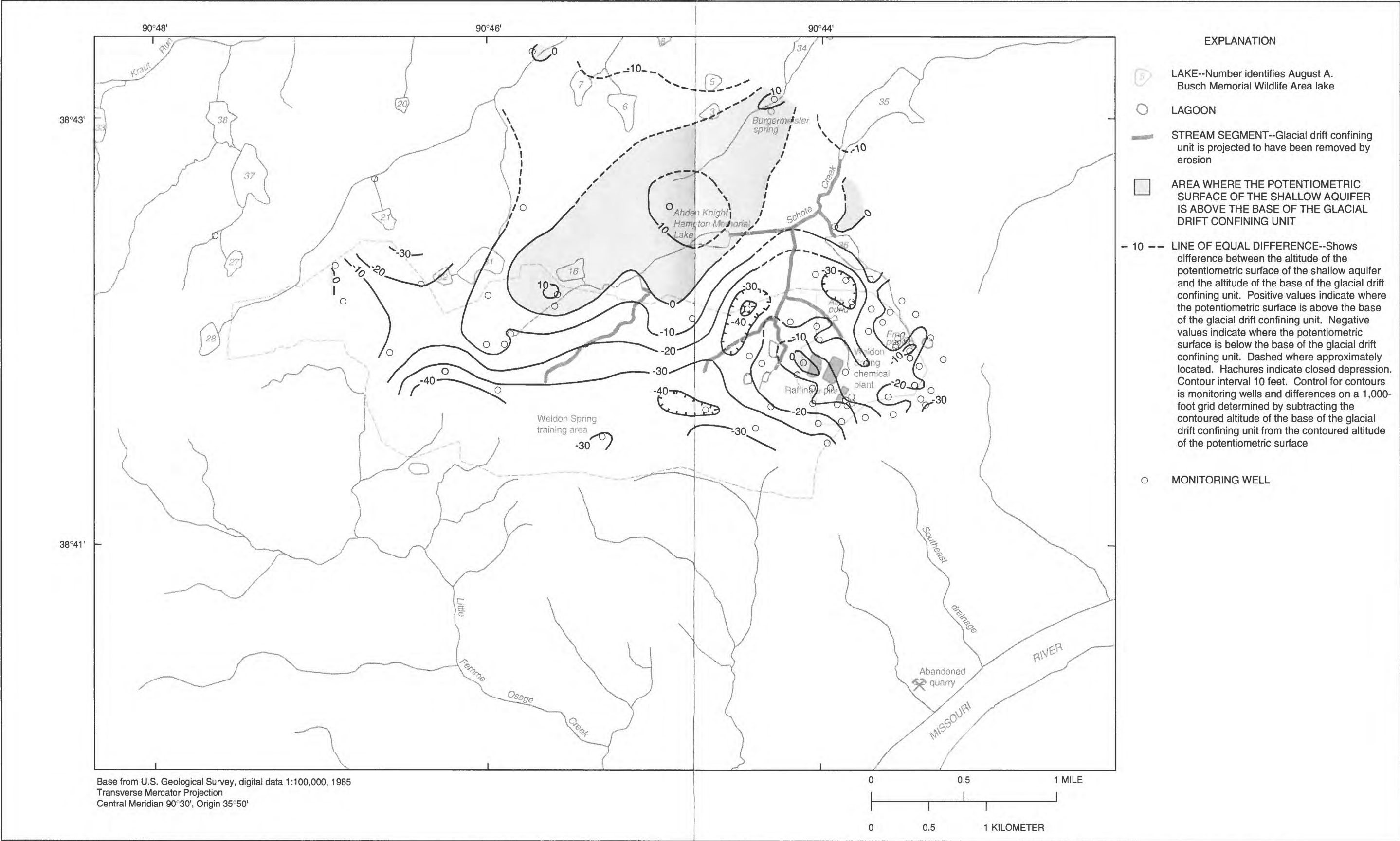
MAP SHOWING THE RELATION OF THE POTENTIOMETRIC SURFACE OF THE SHALLOW AQUIFER AND THE BASE OF THE GLACIAL DRIFT CONFINING UNIT, WELDON SPRING ORDNANCE WORKS, ST. CHARLES COUNTY, MISSOURI
