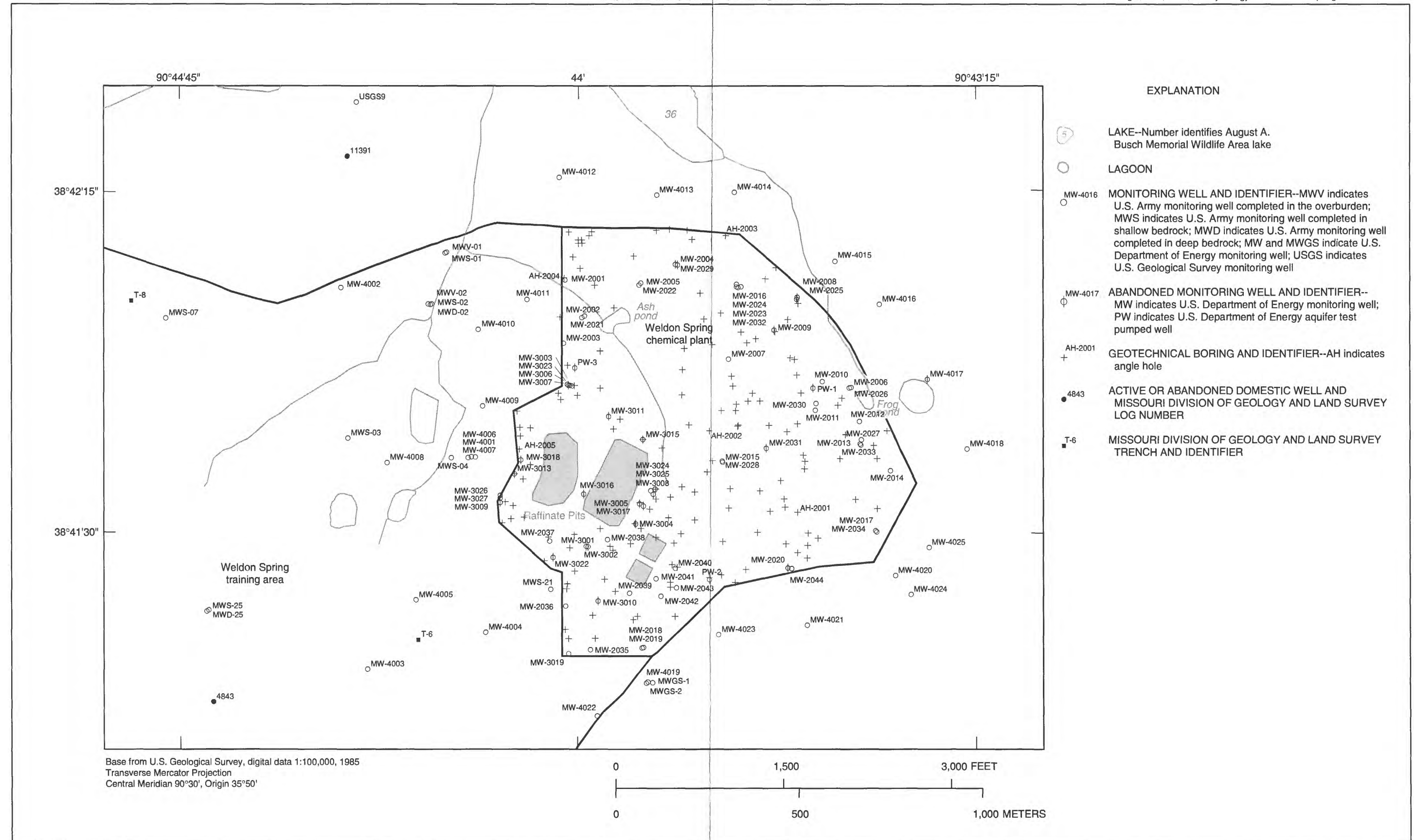
MAP SHOWING LOCATION OF MONITORING WELLS, GEOTECHNICAL BORINGS, DOMESTIC WELLS, AND TRENCHES AT AND IN THE VICINITY OF THE WELDON SPRING CHEMICAL PLANT, ST. CHARLES COUNTY, MISSOURI
