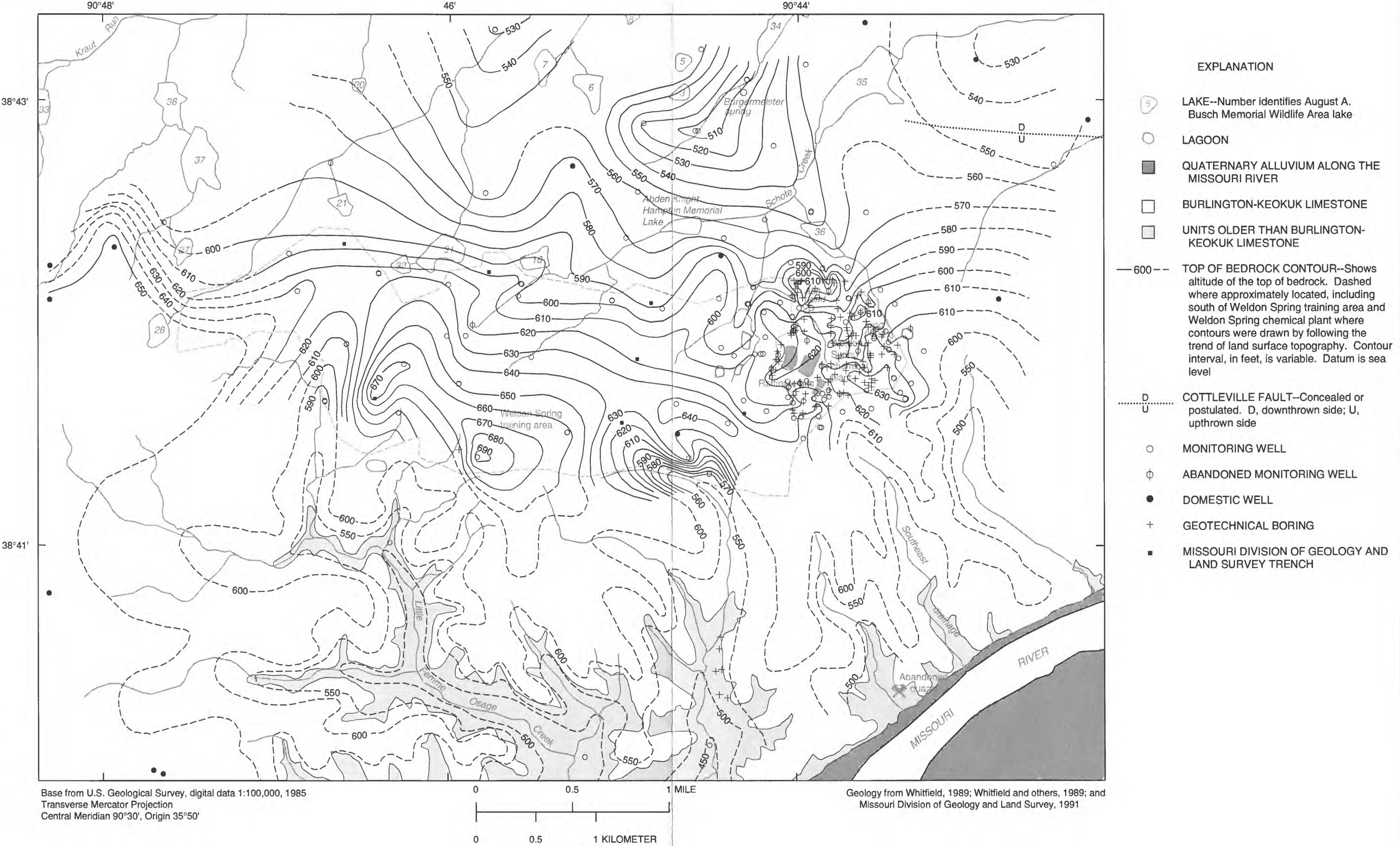
MAP SHOWING ALTITUDE OF THE TOP OF BEDROCK AND GENERALIZED GEOLOGY, WELDON SPRING ORDNANCE WORKS, ST. CHARLES COUNTY, MISSOURI
