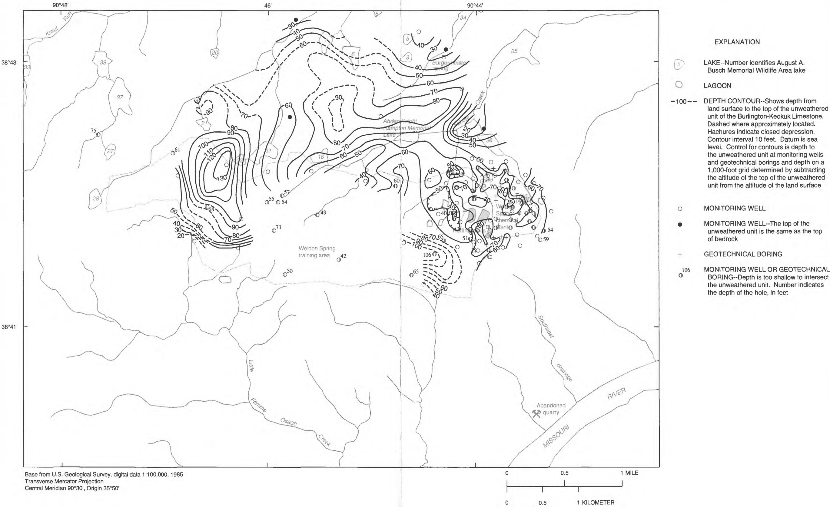
MAP SHOWING DEPTH TO THE TOP OF THE UNWEATHERED UNIT OF THE BURLINGTON-KEOKUK LIMESTONE, WELDON SPRING ORDNANCE WORKS, ST. CHARLES COUNTY, MISSOURI
