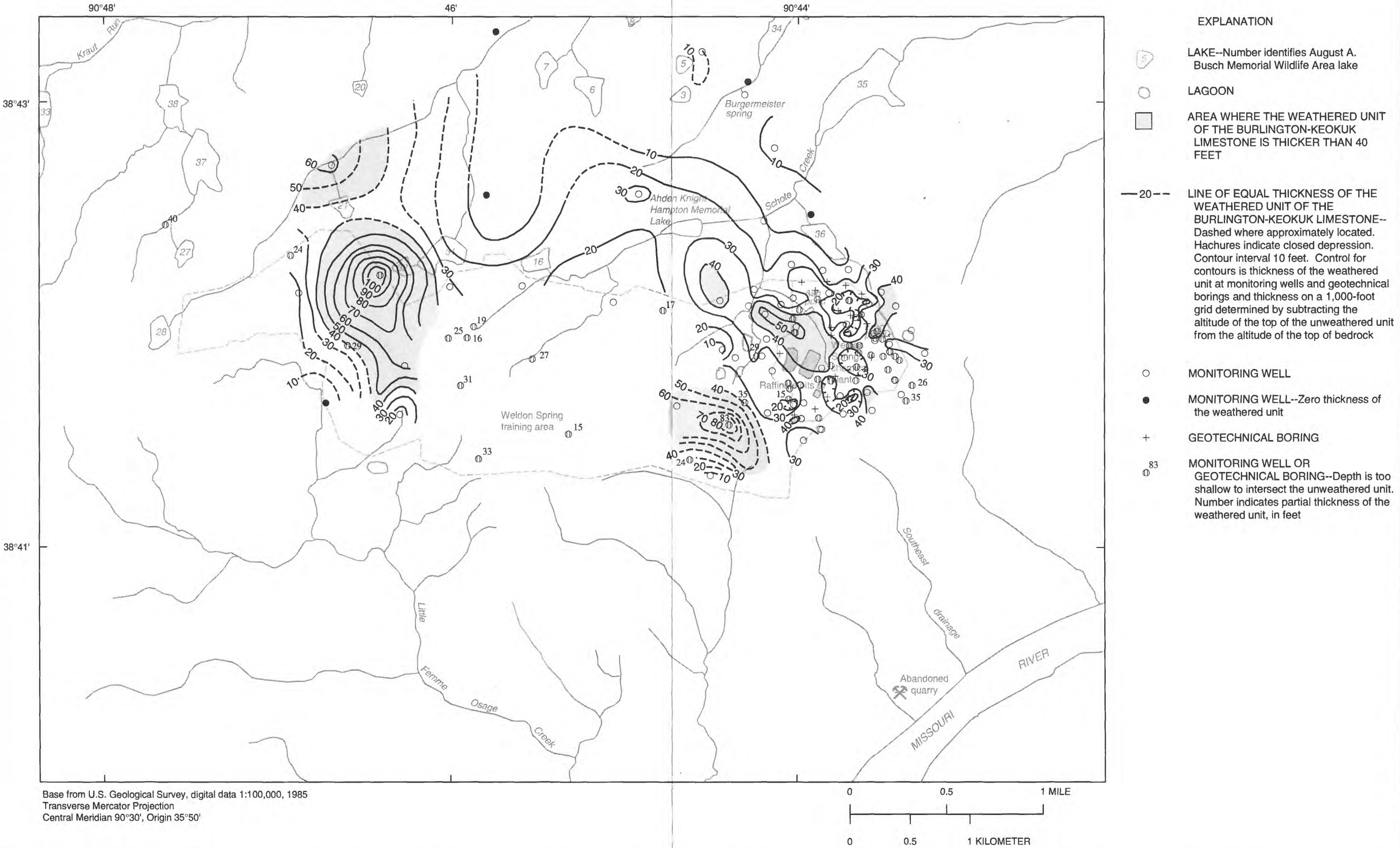
MAP SHOWING THICKNESS OF THE WEATHERED UNIT OF THE BURLINGTON-KEOKUK LIMESTONE, WELDON SPRING ORDNANCE WORKS, ST. CHARLES COUNTY, MISSOURI
