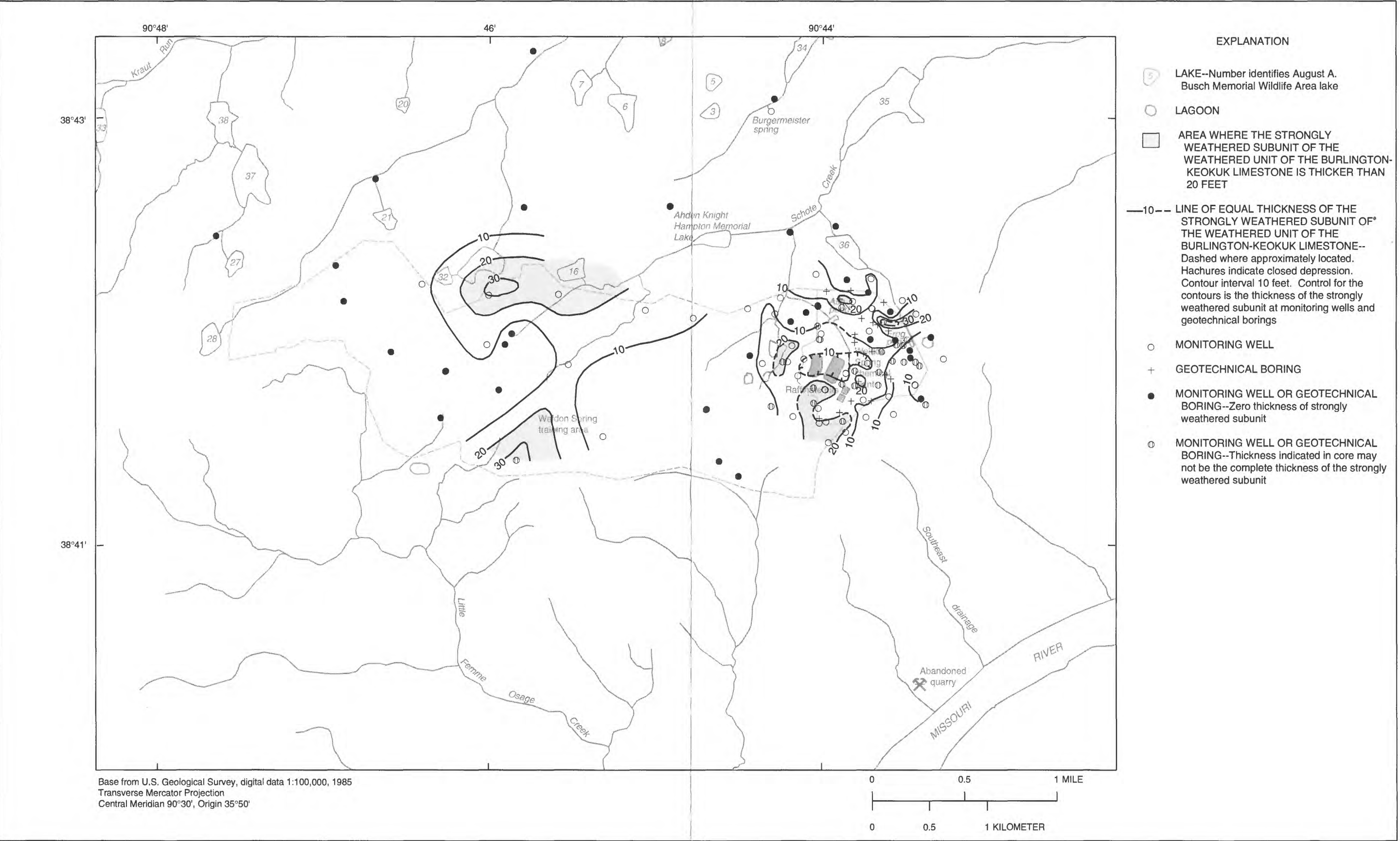
MAP SHOWING THICKNESS OF THE STRONGLY WEATHERED SUBUNIT OF THE WEATHERED UNIT OF THE BURLINGTON-KEOKUK LIMESTONE, WELDON SPRING ORDNANCE WORKS, ST. CHARLES COUNTY, MISSOURI
