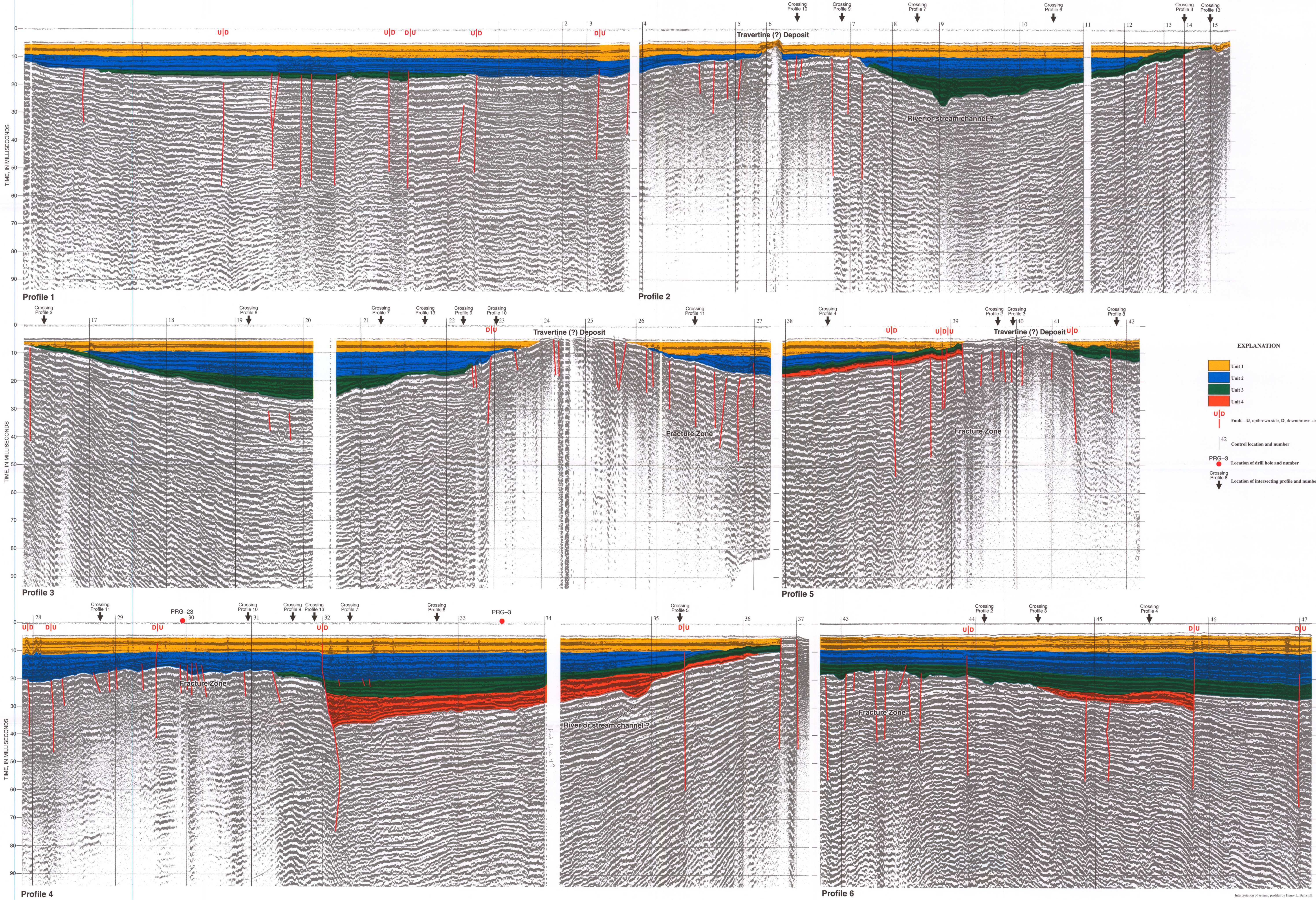
Continuous high-resolution, seismic-reflection profiles 1-6 from the Lincoln Point-Bird Island area, Utah Lake, Utah
