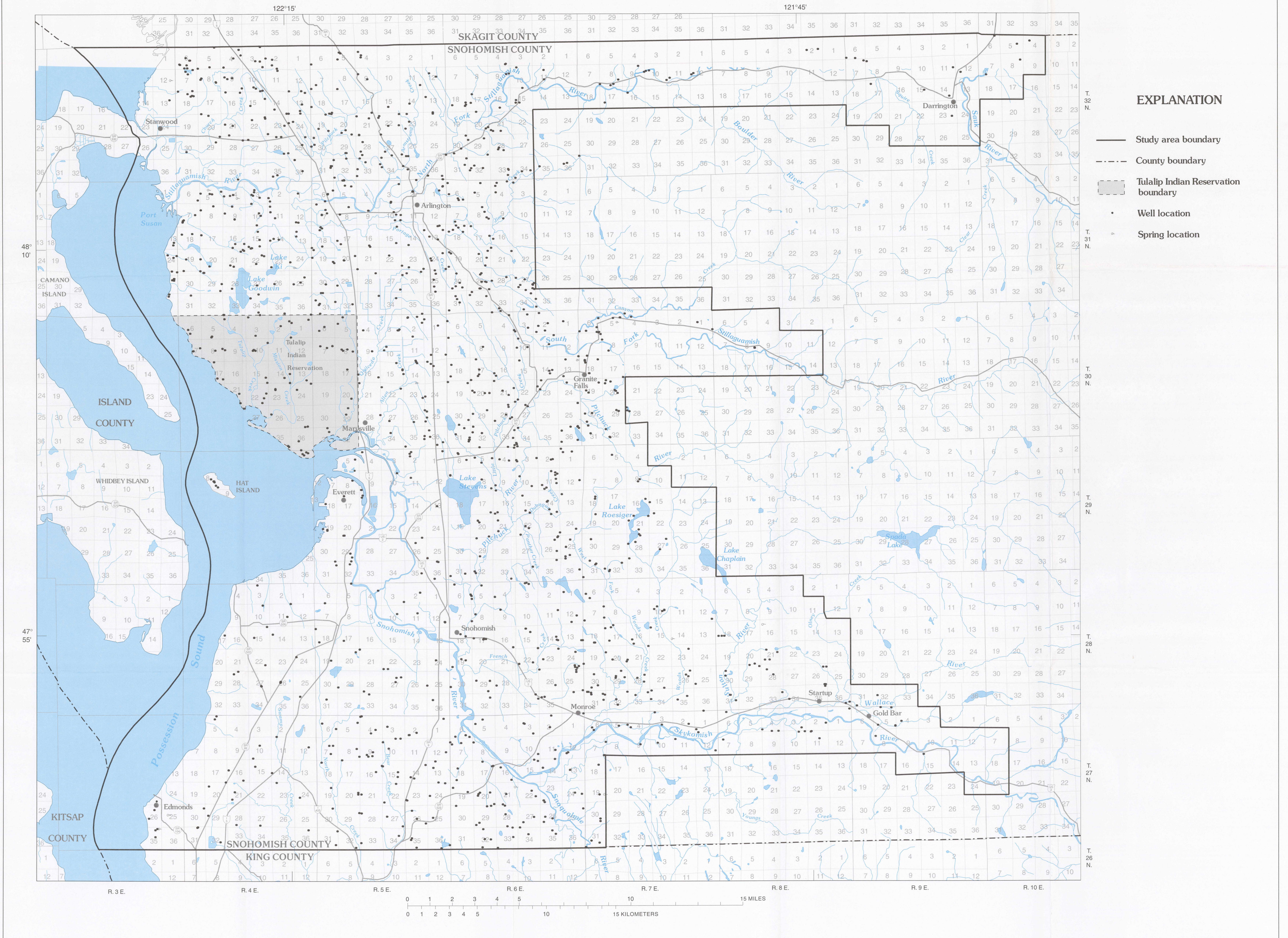
PLATE 1. LOCATIONS OF WELLS AND SPRINGS USED TO COLLECT GEOLOGIC, HYDRAULIC, AND WATER-QUALITY DATA, WESTERN SNOHOMISH COUNTY, WASHINGTON
