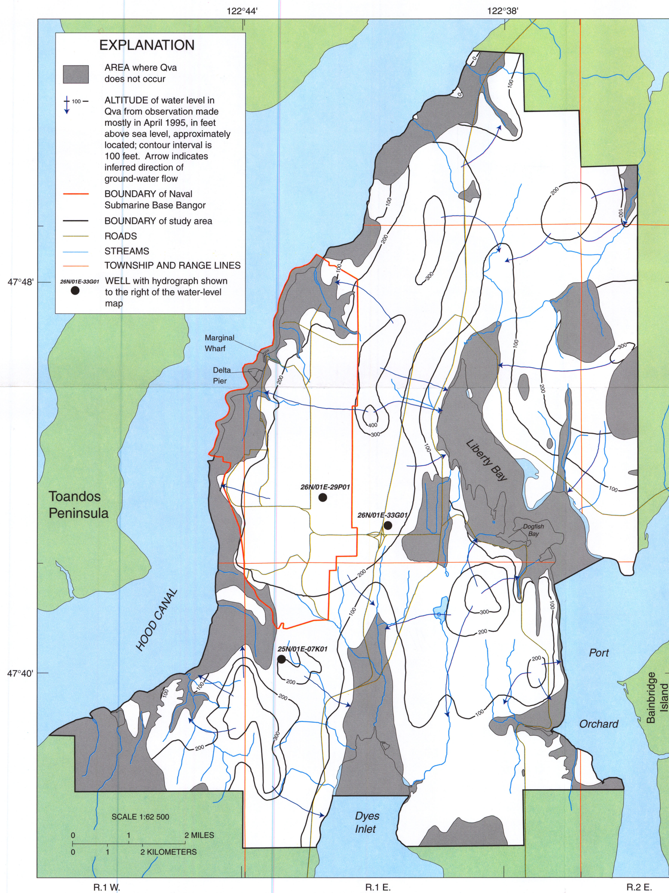
(a) Water levels and inferred directions of ground-water flow, and hydrographs of water levels in selected wells in the Vashon aquifer (Qva)
