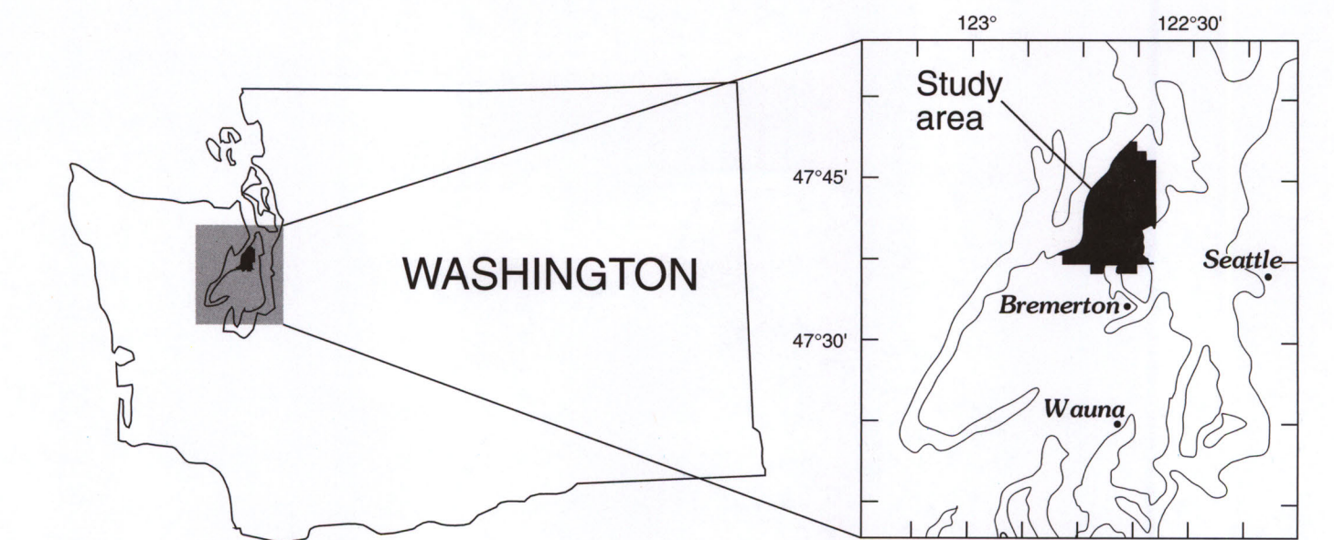
(e) Monthly precipitation measured at Bremerton and Wauna, October 1993 through February 1996, and the locations of Bremerton and Wauna in relation to the study area and Washington State. Data were unavailable for Wauna in April 1994 and for Bremerton in October and December 1994 and January 1995
