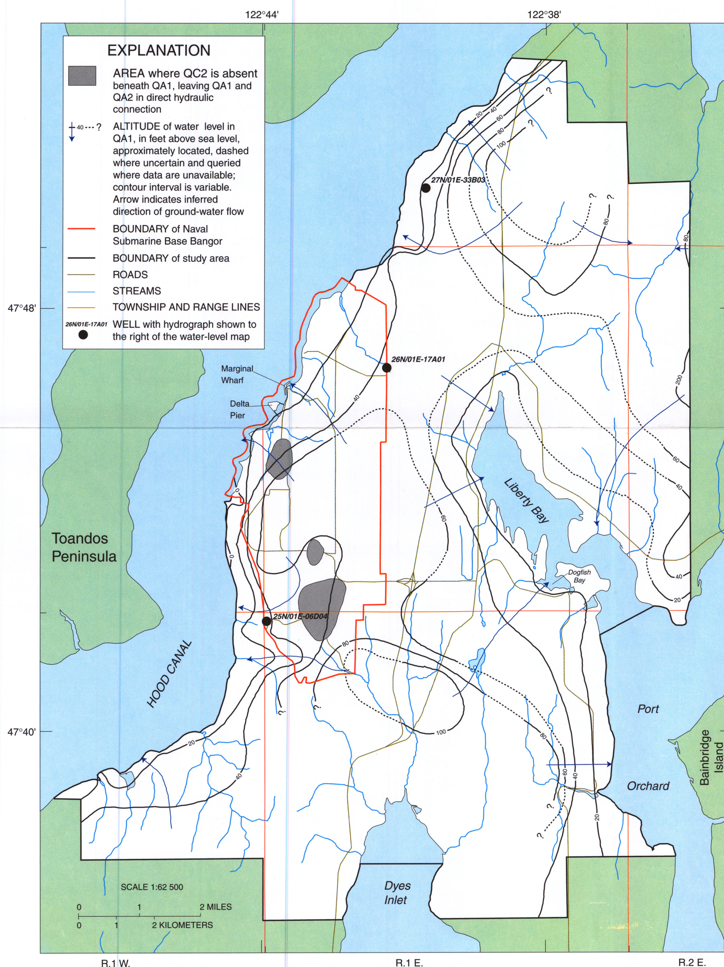
(c) Water levels and inferred directions of ground-water flow, and hydrographs of water levels in selected wells in the Sea-level aquifer (QA1)
