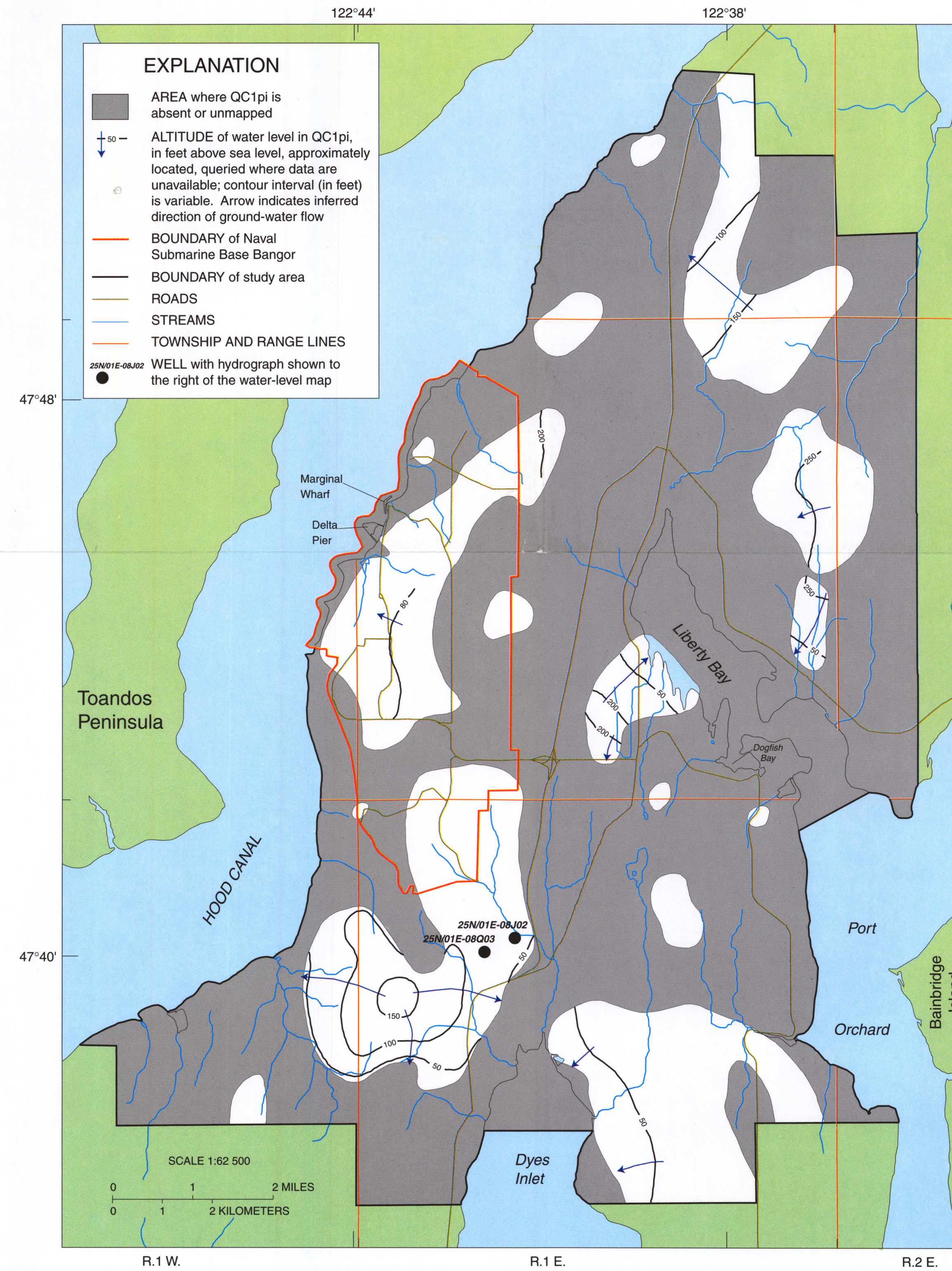
(b) Water levels and inferred directions of ground-water flow, and hydrographs of water levels in selected wells in the Permeable interbeds (QC1pi)
