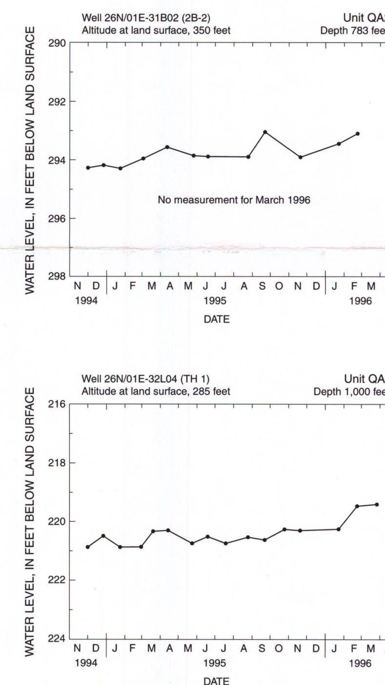
(d) Hydrographs of water levels in selected wells in the Deep aquifer (QA2), see plate 1a for locations of wells
