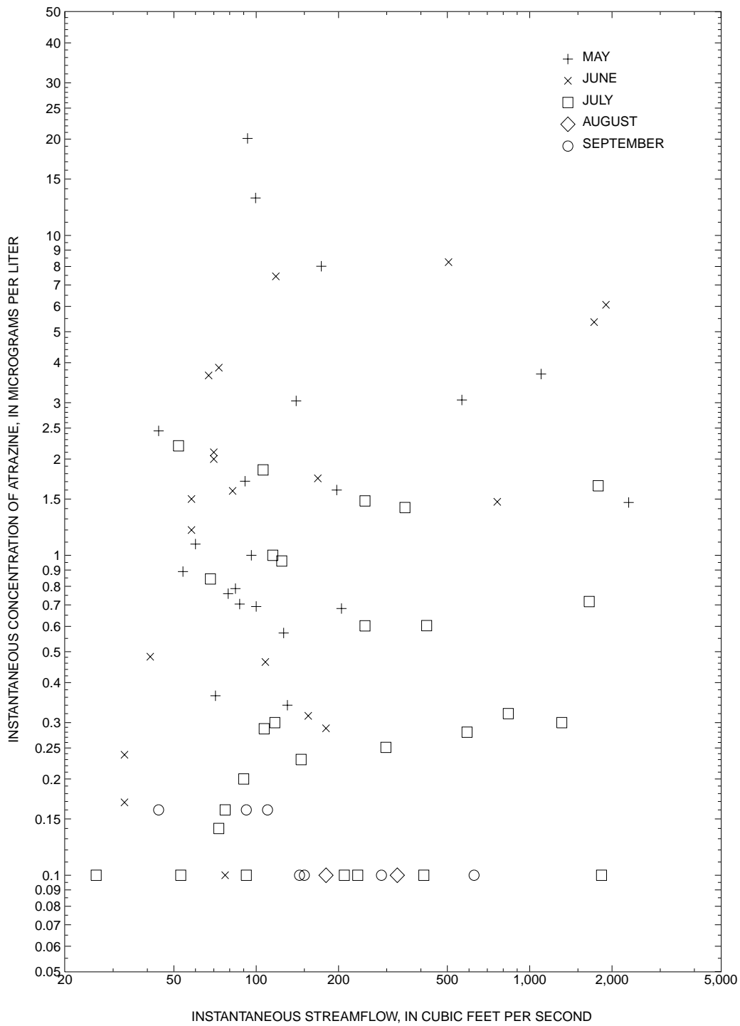
Figure 5. Relation between streamflow and atrazine concentration during periods of stormflow, May to September, 1992 through 1995, Mill Creek at Elshelman Mill Road near Lyndon, Pennsylvania.
